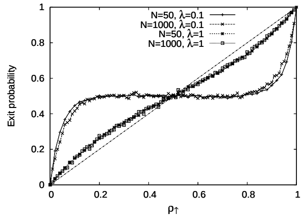
FIG. 2: Exit probability \mathcal{E}(\rho_{\uparrow}) versus the density of \uparrow voters \rho_{\uparrow} for N = 50 and N = 1000 , in the case of a one-dimensional system. The exit probability has a non-trivial dependence on the initial condition, with a trend toward zero magnetization. When \lambda is decreased, the dynamics loses its dependence on the initial conditions and \mathcal{E}(\rho_{\uparrow}) = 1/2 .
