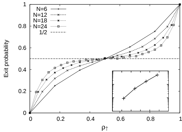
FIG. 1: Exit probability \mathcal{E}(\rho_{\uparrow}) versus the density of \uparrow voters \rho_{\uparrow} for N = 6 , N = 12 , N = 18 and N = 24 in the mean-field case. In the inset, we plot the average time to reach consensus as a function of N on a log scale. Simulation results are averaged over 5000 realizations of the random process.
