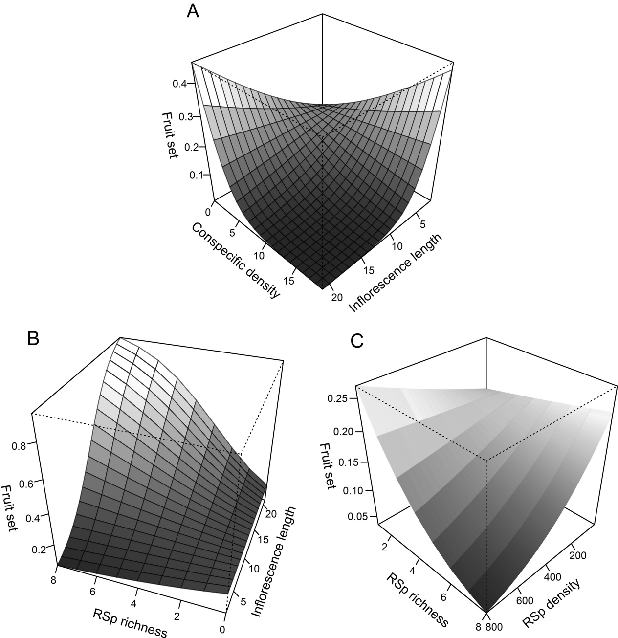
Figure 4 – Interaction surface plots: A, fruit set in Orchis militaris in relation to O. militaris inflorescence length and conspecific density; B, fruit set in O. militaris in relation to O. militaris inflorescence length and species richness of co-flowering rewarding species (RSp richness); C, fruit set in O. militaris in relation to density of co-flowering rewarding species (RSp density) and RSp richness.
