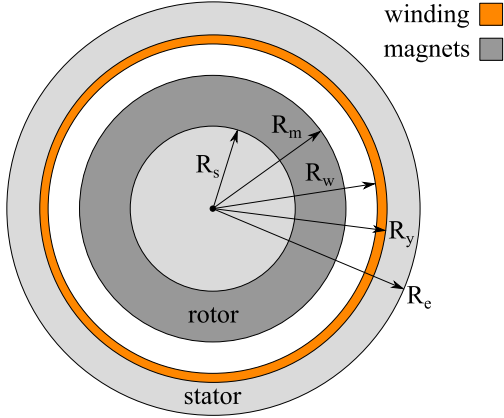
Fig. 1. Bearing topology and design parameters.
