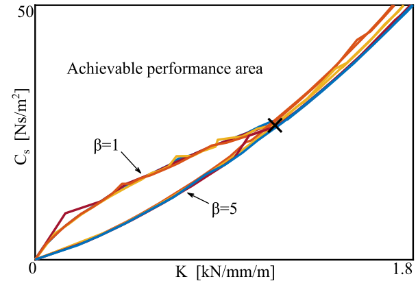
Fig. 8. Zoom on the area of interest where C_s < 50 Ns/m.
