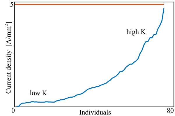
Fig. 4. Current densities associated with the individuals on the Pareto front, and maximum value of 5 A/mm 2 .
