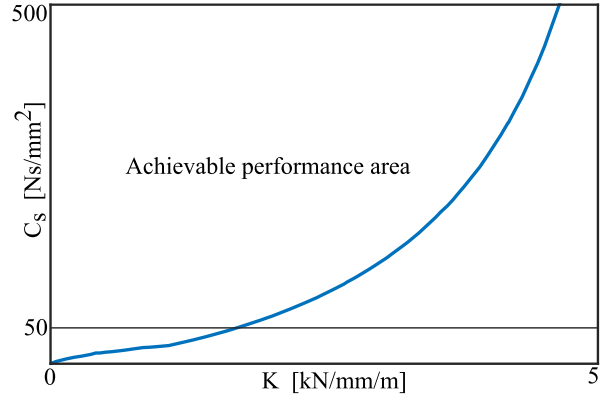
Fig. 3. Pareto front of the bearing performance at \omega = 2\pi 1000 rad/s.
