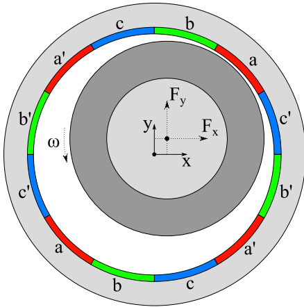
Fig. 2. Rotor position, electrodynamic forces and winding phases.
