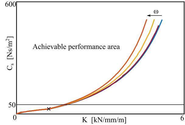
Fig. 7. Pareto fronts for \omega = 2\pi\{50, 100, 500, 1000\} rad/s.
