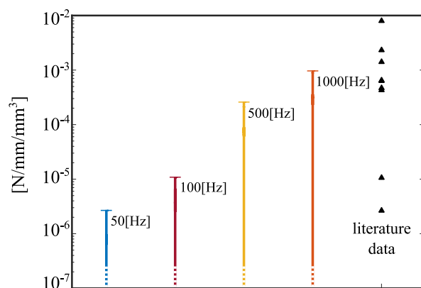
Fig. 9. Stiffness to volume ratio of the existing EDBs (triangles) and of the individuals on the Pareto fronts of Fig. 7 (solid lines).
