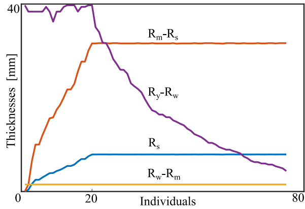
Fig. 6. Width of the shaft ( R_s ), PMs ( R_m - R_s ), air gap ( R_w - R_m ) and winding ( R_y - R_w ).
