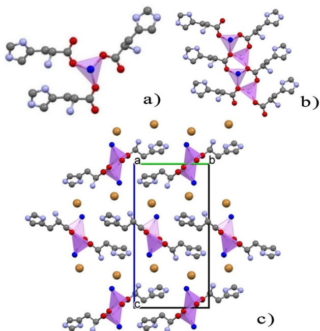
Figure 1. L-His · LiBr · H 2 O (CSD refcode AZIPOQ [33] ). (a) Tetrahedral coordination around the Li + cation; (b) portion of the infinite chain of lithium coordination tetrahedra; (c) crystal packing. Water oxygens in blue; Li + coordination polyhedra in lilac; bromide ions in brown; hydrogen atoms omitted for clarity.
