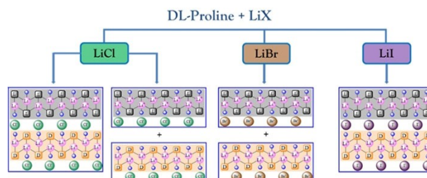
Scheme 2. CocrySTALLIZATION of DL-proline with lithium halides. “L” and “D” stay for L- and D-proline respectively; blue spheres represent water oxygens.
