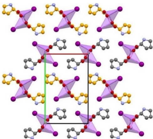
Figure 5. The crystal packing arrangement of DL-Pro·Lil (CSD refcode MISKEH [35] ). Grey and orange spheres for carbons refer to proline molecules with opposite chirality; Li + coordination polyhedra in lilac; iodide ions in purple; H atoms omitted for clarity.
