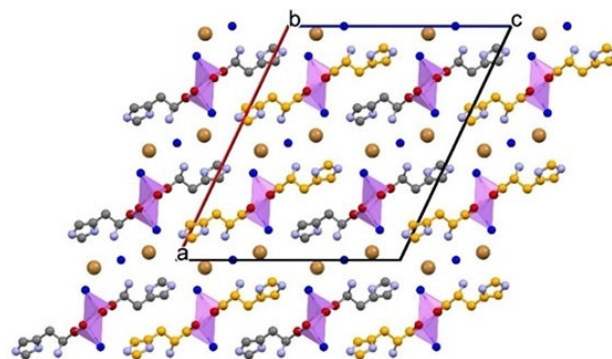
Figure 2. Crystal packing of DL-His · LiBr · 1.5H 2 O (CSD refcode AZIPIK [33] ). Water oxygens in blue; grey and orange spheres for carbons ETI 2 · CaCl 2 · 2H 2 O refer to histidine molecules with opposite chirality; Li + coordination polyhedra in lilac; bromide ions in brown; Hydrogen atoms omitted for clarity.
