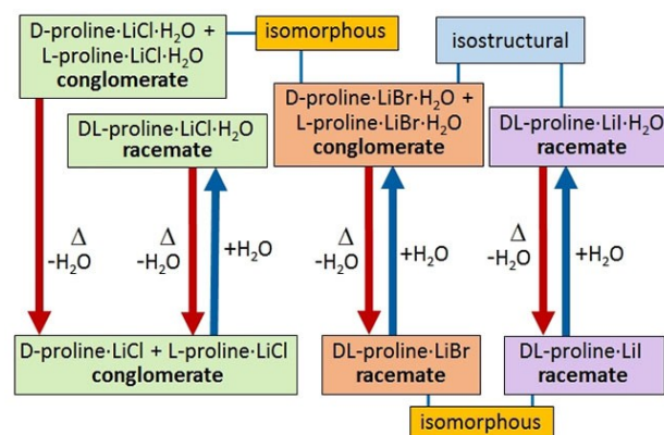
Scheme 3. Dehydration/rehydration processes involving all the hydrated ICCs containing both L- and D-proline enantiomers; structural relationships between isomorphous pairs indicated in yellow. Reproduced from Ref. [35] with permission from Wiley.
