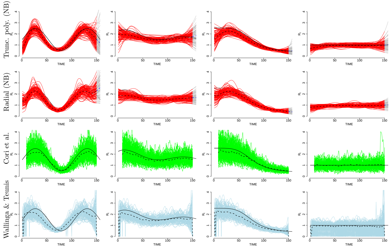
Fig. 2. Spline-based estimated R(t) using truncated polynomial or radial bases and a negative binomial (NB) distributional assumption. The estimates for 100 different simulated epidemics are shown in each panel. The solid black line depicts the true R(t) function, the solid coloured lines depict the 100 different estimates, while the dotted lines depict the empirical averages over the 100 estimates at each time point. The estimates based on the methods of Cori et al. (2013) and Wallinga and Teunis (2004) are also presented. For the spline-based method we also show the 7-day ahead forecasts for R(t) .
