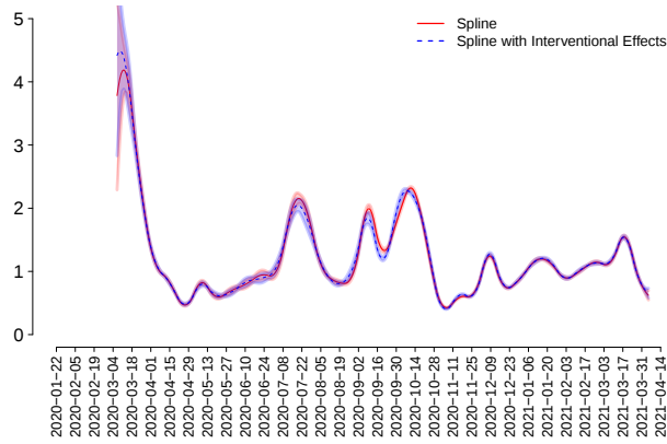
Fig. 5. Spline-based estimated R(t) with 95% pointwise confidence interval for Belgium. The estimator accounting for the interventions (dashed line) is presented alongside the estimator that does not account for interventions (full line).
