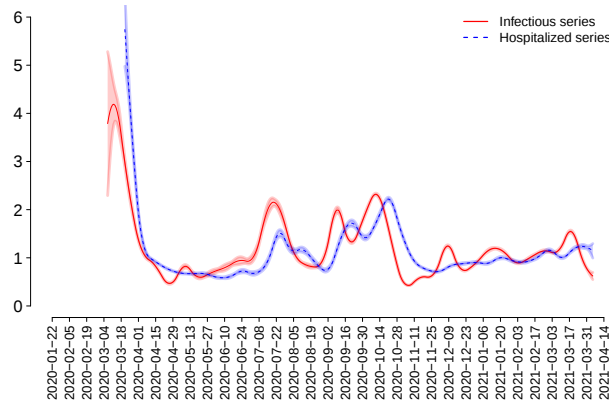
Fig. 7. Spline-based estimated R(t) with 95% pointwise confidence interval for Belgium. The estimator based on the 7-day moving average data of the hospitalized series (dashed line) is presented alongside the estimator that uses the 7-day moving average of the infectious series (full line).
