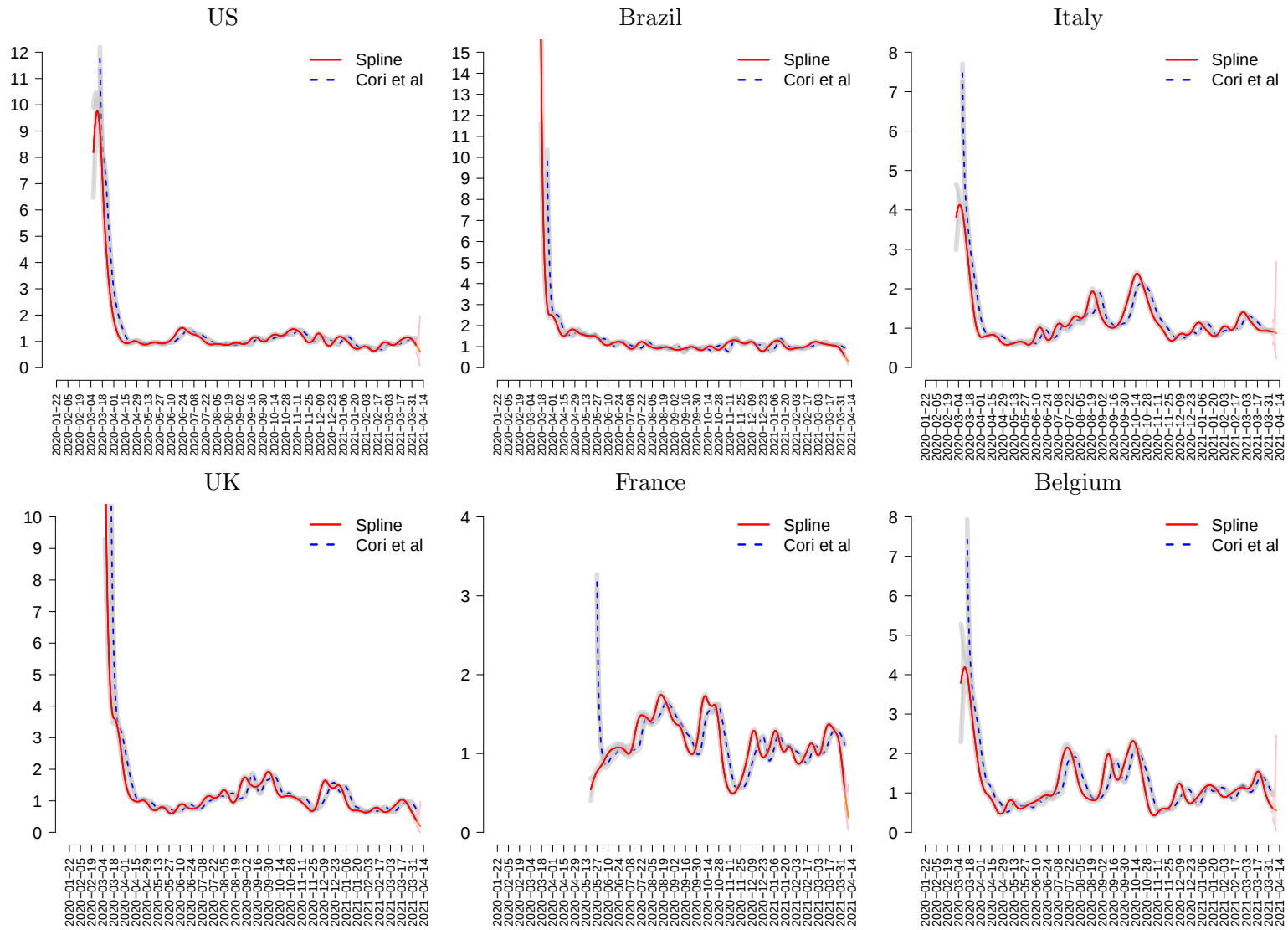
Fig. 4. Spline-based estimated R(t) (and 95% pointwise confidence interval) using truncated polynomial bases and a negative binomial assumption for six countries. The evolution 5-days ahead (ie. for the period 6-10th of April, 2021) together with a simulation-based prediction interval is also presented. The estimates based on the method of Cori et al. (2013) are also presented.
