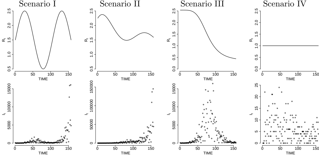
Fig. 1. Simulated data from four different scenarios. Top panels correspond to different R(t) functions while the bottom panels represent counts of infections I(t) simulated from models corresponding to each R(t) .
