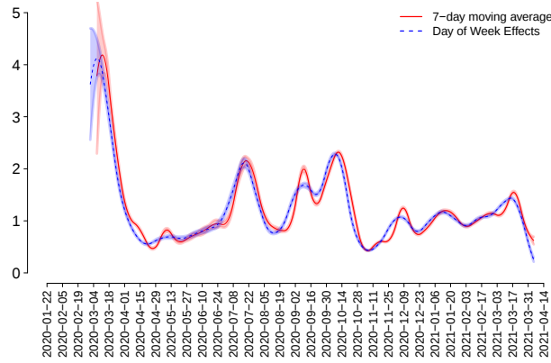
Fig. 6. Spline-based estimated R(t) with 95% pointwise confidence interval for Belgium. The estimator accounting for the day of the week and using the raw data (dashed line) is presented alongside the estimator that uses the 7-day moving average data (full line).
