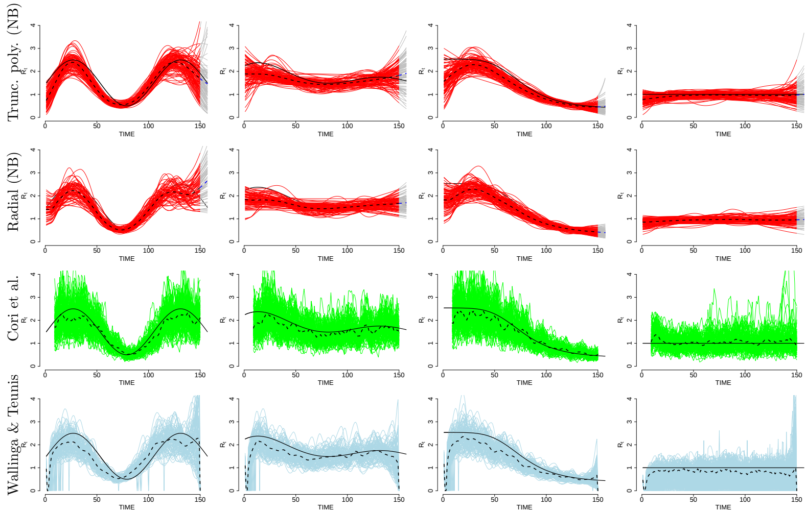
Fig. 3. Spline-based estimated R(t) using truncated polynomial or radial bases and a negative binomial (NB) distributional assumption. The estimates for 100 different simulated epidemics are shown in each panel obtained when there is between 50-70% under-reporting in the data for each day. The solid black line depicts the true R(t) function, the solid coloured lines depict the 100 different estimates, while the dotted lines depict the empirical averages over the 100 estimates at each time point. The estimates based on the methods of Cori et al. (2013) and Wallinga and Teunis (2004) are also presented. For the spline-based method we also show the 7-day ahead forecasts for R(t) .
