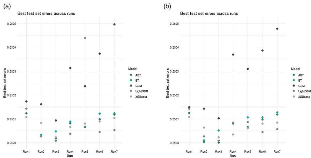
Figure 6. Minimal test set deviance for each run. (a) Validation set. (b) Cross-validation.
