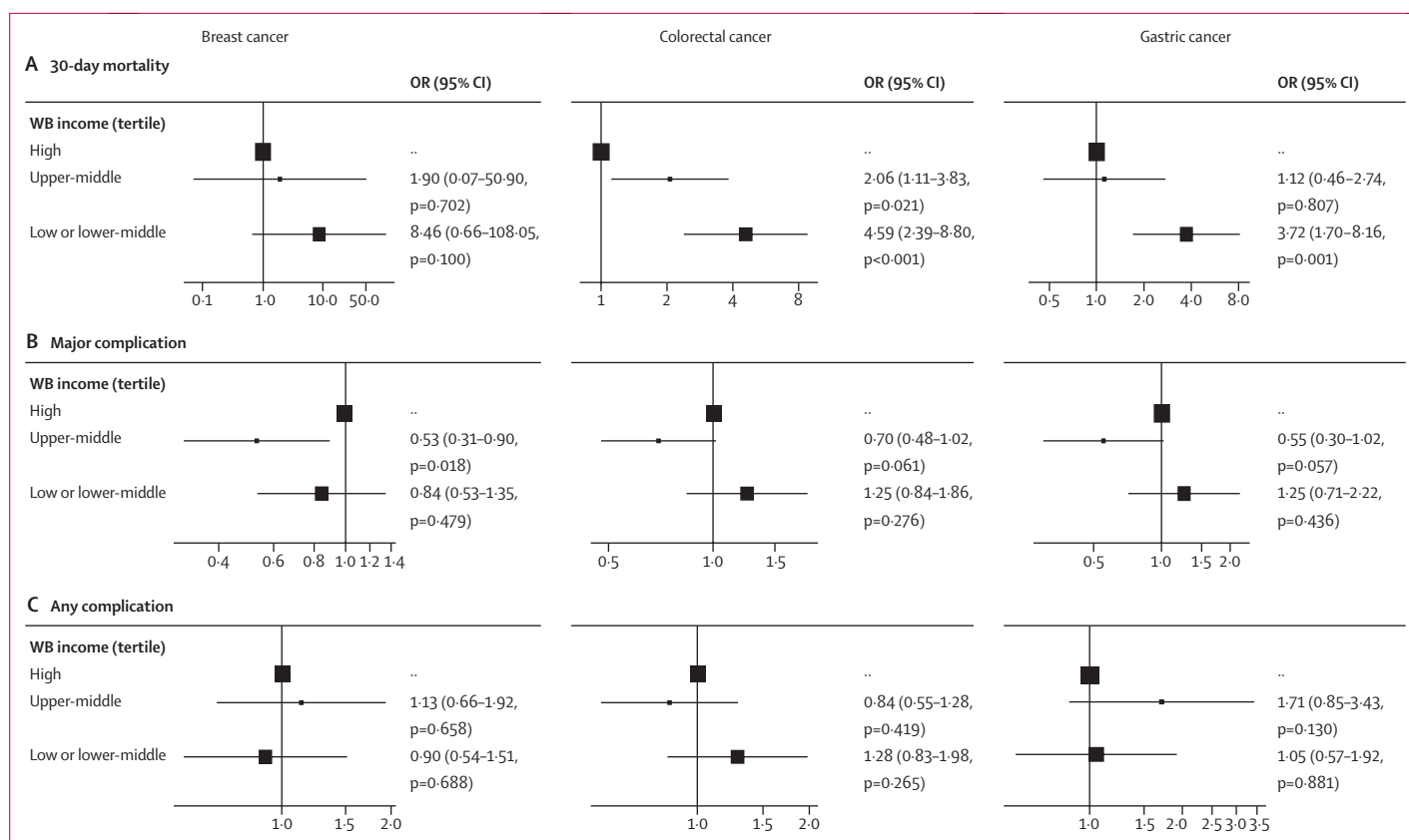
Figure 4: Multilevel logistic regression-adjusted outcomes by World Bank country income group
