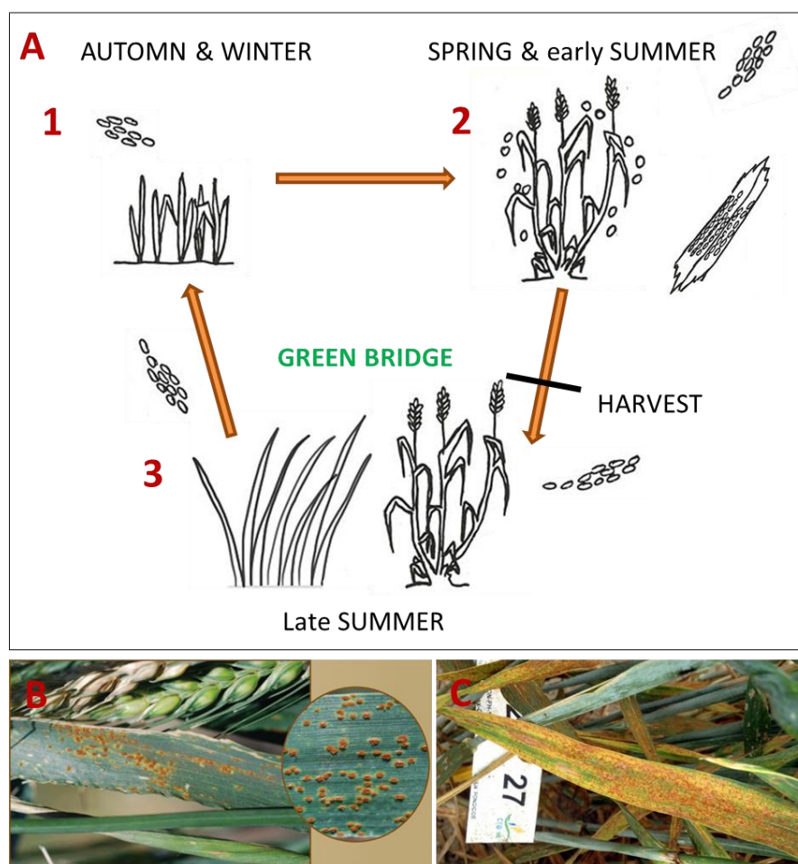
Figure 1.3. A) Asexual cycle of WLR caused by Puccinia triticina . A1) In autumn, urediniospores contaminate young plants in a new crop from volunteer wheat plants and the pathogen then overwinters on these plants. A2) Secondary cycles of infection occur under favorable conditions. Depending on the temperature, a full asexual cycle can be completed in 8-12 days. Infection spread within a crop occurs rapidly by wind and contact, and can also occur with spores coming from distant infected fields. A3) After harvesting, urediniospores are produced on volunteer, leading to the infection of wheat crops in the following season. This phenomenon is called the 'green bridge'. B&C) Typical WLR symptoms on the upper leaves of wheat. The fungus forms small reddish-orange pustules (uredinia), which rupture the upper surface of the leaf blade as the spores mature. Individual pustules are circular to oval, with a diameter of 1.5 mm.
