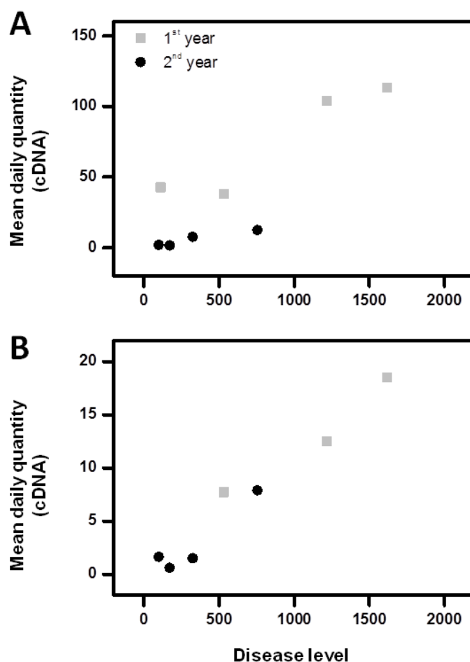
Figure 2. 7. Disease level values for untreated plants of a given crop in relation to the mean daily airborne inoculum quantities trapped over two periods: A , from stem elongation (mid-April) to the beginning of harvest (31 July); and B , from 1 September to stem elongation of the next crop. Grey squares represent the data for the first year of trapping and black circles represent data for the second year of trapping. On the figure B, one point was removed because the spore trap was moved to a new field 15 km away in October 2011, without any knowledge of the STB disease level in the previous wheat crop in this new field.
