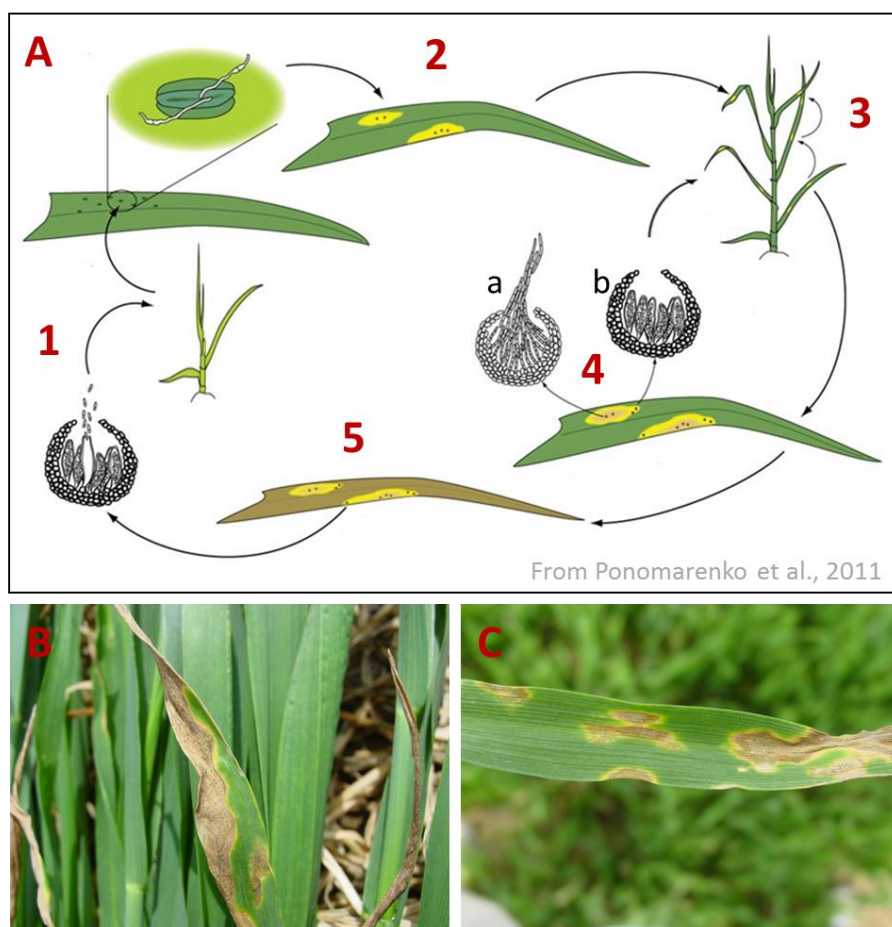
Figure 1.2. A) Disease cycle of STB caused by Mycosphaerella graminicola . A1) In a crop rotation system, the primary infection of plants is caused mainly by airborne ascospores produced on residues of previous wheat crops. Ascospores contaminate young plants through leaf stomata. A2) First lesions on young plants develop pycnidia. A3) Secondary spread of pycnidiospores (vertical and horizontal dispersal) caused by contact and rain dispersal. A4a) Pycnidia that have developed on lesions produce great quantities of pycnidiospores throughout the growing season. A4b) Pseudothecia develop on lesions, releasing mobile airborne ascospores that can contaminate wheat plants. 5) Pathogens overwinter as mycelia, pycnidia, pseudothecia on crop debris and on autumn-sown crops and volunteer hosts. B & C) Typical STB symptoms on an upper leaf of winter wheat
