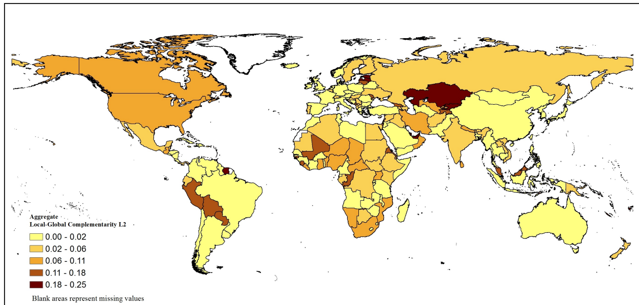
Figure C.5. Local-Global Complementarity by Country – Level 2
