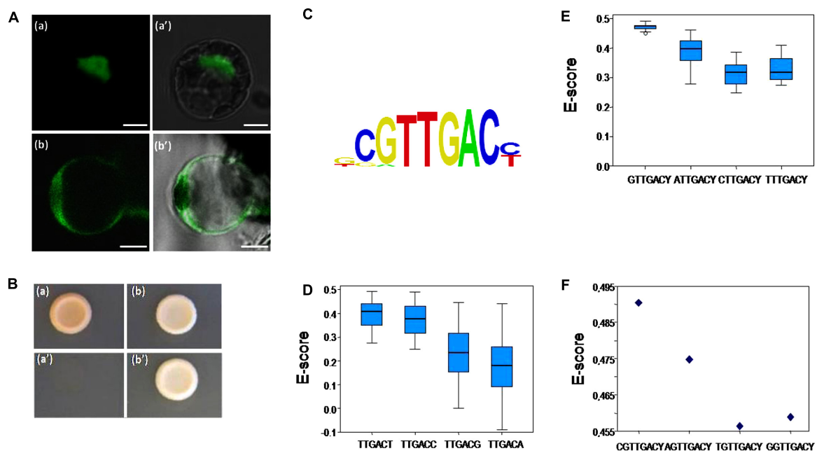
FIGURE 2 | SIWRKY3 subcellular localization, trans -regulation properties and DNA-binding specificities. (A) Transient expression of YFP-SIWRKY3 fusion protein and control YFP in tomato leaf protoplasts. (a,a') YFP-SIWRKY3 fluorescence and bright field/YFP fluorescence, respectively. (b,b') Control YFP fluorescence and bright field/YFP fluorescence, respectively. Scale bar indicates 5 \mu M. (B) SIWRKY3 transactivation ability. SIWRKY3 coding region was fused to GAL4-DBD into the pGBKT7 vector carrying the nutritional marker TRP1 as reporter gene. The resulting plasmid, and the empty pGBKT7 vector used as negative control, were transformed into the yeast strain Y8930 harboring ADE2 and HIS3 reporter genes. Yeasts were separately grown on SD (synthetic dropout) medium lacking either tryptophan (a,b; pGBKT7 or GAL4-DBD-SIWRKY3, respectively), or adenine and histidine (a',b'; pGBKT7 or GAL4-DBD-SIWRKY3, respectively). (C) Position weight matrix (PWM) representation of the top scoring 8-mer obtained in "seed-and-wobble" algorithm. (D) Box plot of the distribution of enrichment scores ( E -scores) of all possible 8-mers containing the indicated elements. Boxes represent quartiles 25–75%, black line represents the median of the distribution (quartile 50%) and bars indicate quartiles 1 to 25% (above) and 75 to 100% (below). The higher and sharper distributions of E -scores corresponding to TTGACT and TTGACC motifs reflect higher binding affinity of SIWRKY3 to these elements. (E) Box plot of the distribution of E -scores of all possible 8-mers containing the indicated elements varying at their 5'-end nucleotide, showing highest affinity of SIWRKY3 for the DNA element GTTGACY. Representation of the boxes is as in (D) . (F) E -scores of the 8-mers indicated in the Figure. Each point represents the average of two different E -scores, corresponding to NGTTGACC and NGTTGACT. Highest affinity was observed for CGTTGACY, as represented in the logo representation in (C) . In spite of this, all the 8-mers containing the element GTTGACY were very efficiently recognized by SIWRKY3.
