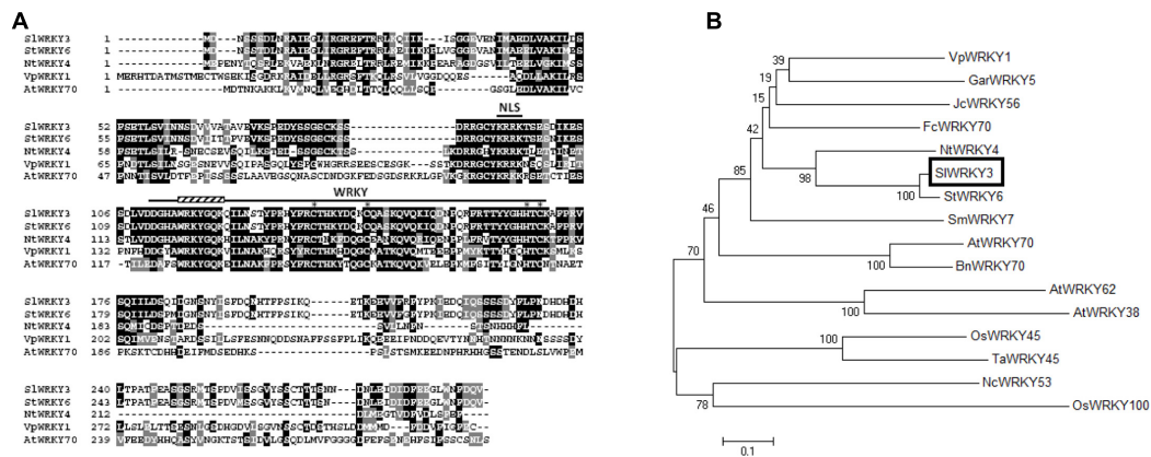
FIGURE 1 | Identification of SIWRKY3. (A) Comparison of SIWRKY3 sequence with StWRKY6, NtWRKY4, VpWRKY1, and AtWRKY70. Identical residues are colored in black, and conserved residues in dark gray. The WRKY domain and the putative nuclear localization site are labeled. The Cys and His residues forming the zinc-finger motif are indicated by stars. (B) Phylogenetic analysis of SIWRKY3 and related proteins: StWRKY6, NtWRKY4, GarWRKY5, JcWRKY56, FcWRKY70, SmWRKY7, VpWRKY1, AtWRKY70, AtWRKY62 and AtWRKY38, NcWRKY53, BnWRKY70, OsWRKY45, OsWRKY100, and TaWRKY45. The phylogenetic tree was constructed according to the neighbor-joining method, using MEGA6 (Tamura et al., 2013). The percentage of reliability of each branch point of the rooted tree, as assessed by the analysis of 1000 trees (bootstrap replicates), is shown on the branch stem.
