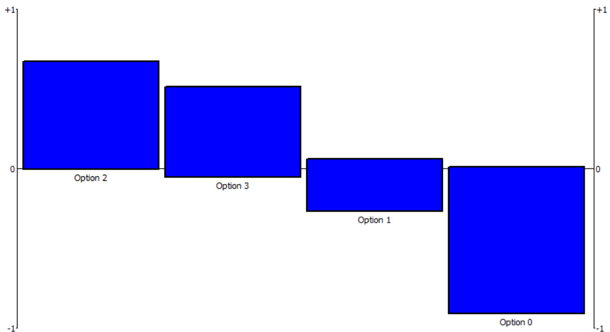
Figure 6 - Net flows of the alternatives for specification of MAT (basic weighting scenario)
