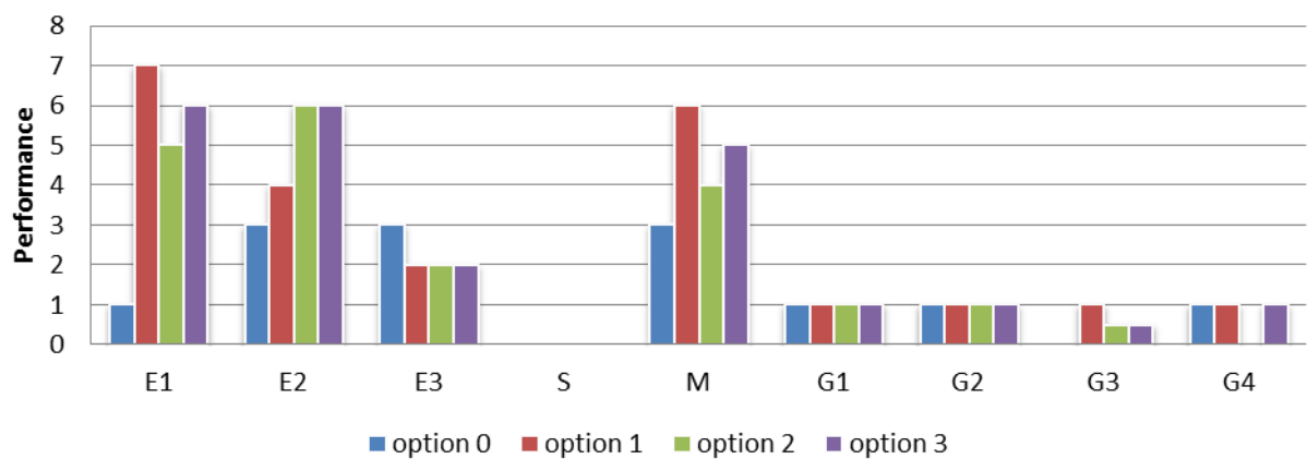
Figure 3 - Performance chart of the options for the operationalization of PIC
