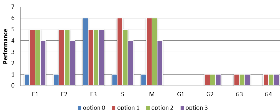
Figure 11 – Performance chart of the alternatives for the ABS CH
