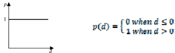
Figure 2 - Usual preference function
