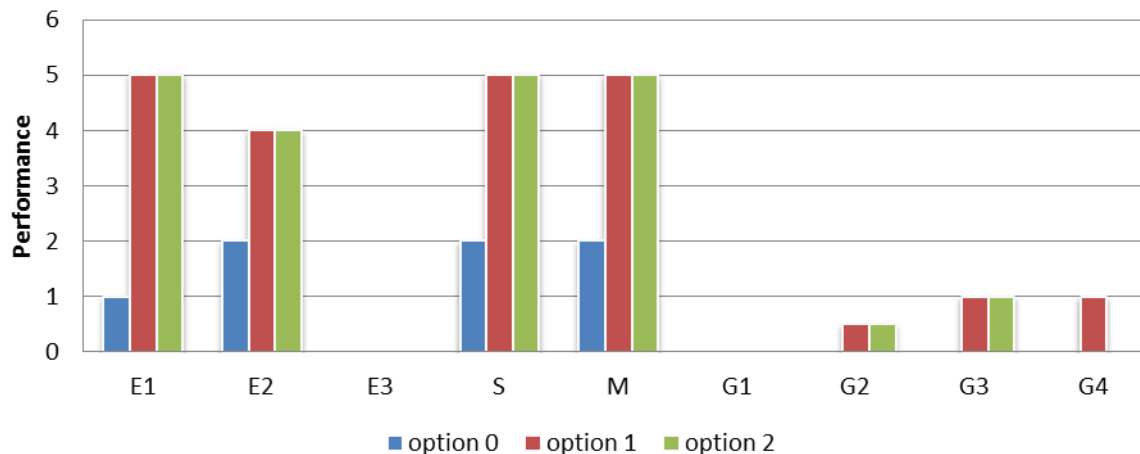
Figure 8 - Performance chart for the options setting up compliance measures
