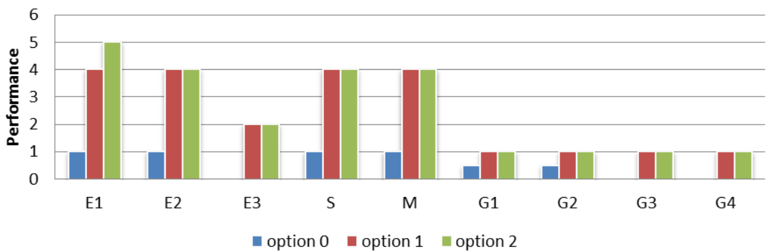
Figure 7 - Performance chart for the establishment of the CNA
