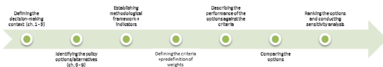
Figure 1 - Steps of the MCA
