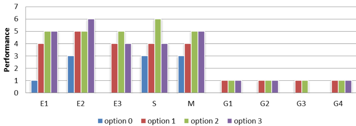
Figure 5 - Performance chart of the options for the specification of MAT
