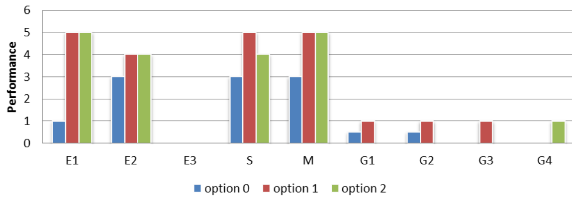
Figure 10 - Performance chart for the options designating checkpoints
