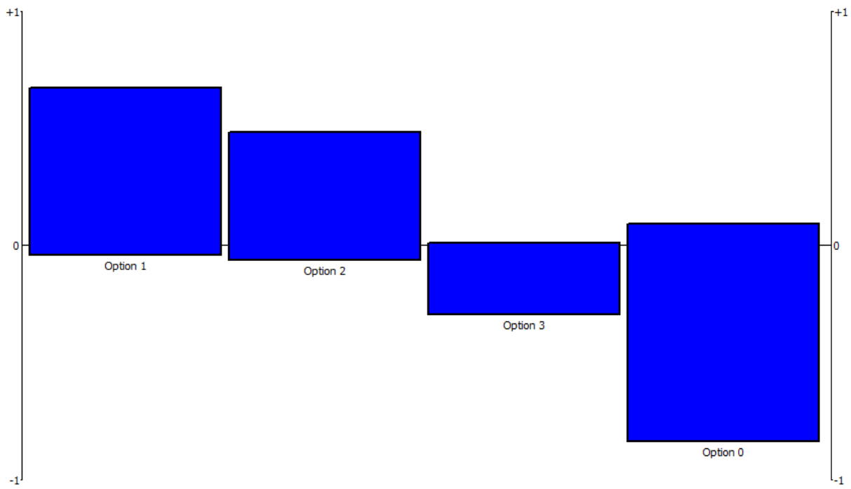
Figure 12 - Net flows of the alternatives for the ABS CH (basic weighting scenario)
