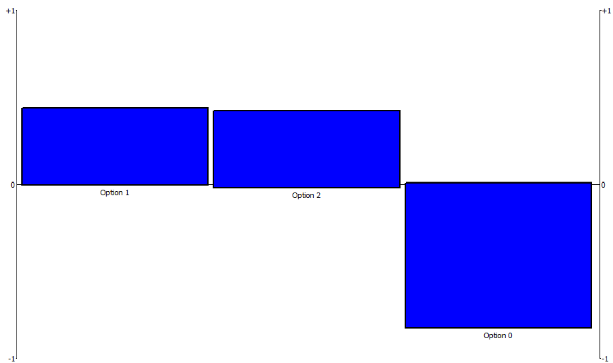
Figure 9 - Net flows of the alternatives for setting up compliance measures (basic weighting scenario)
