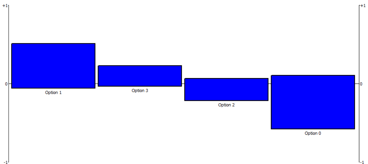
Figure 4 - Net flows of the alternatives for operationalizing PIC (basic weighting scenario)
