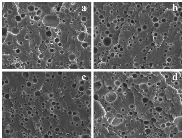
Fig. 4 SEM micrographs of (a) unfilled PA11/PEO, and blends containing (b) C15A, (c) C30B and (d) C-Na + .
