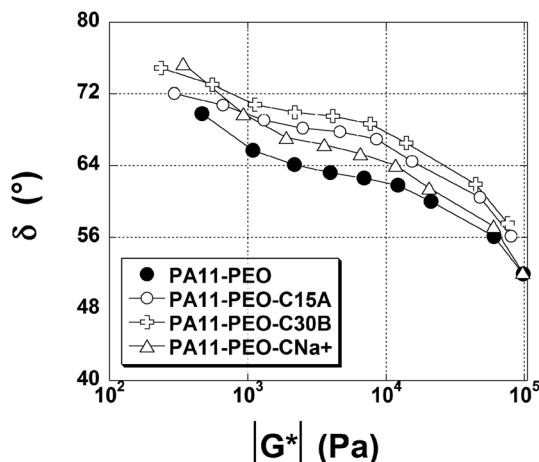
Fig. 10 van Gurp–Palmen plot (phase angle, \delta , versus absolute complex modulus, |G^*| ) of the unfilled and clay-based PA11/PEO.
