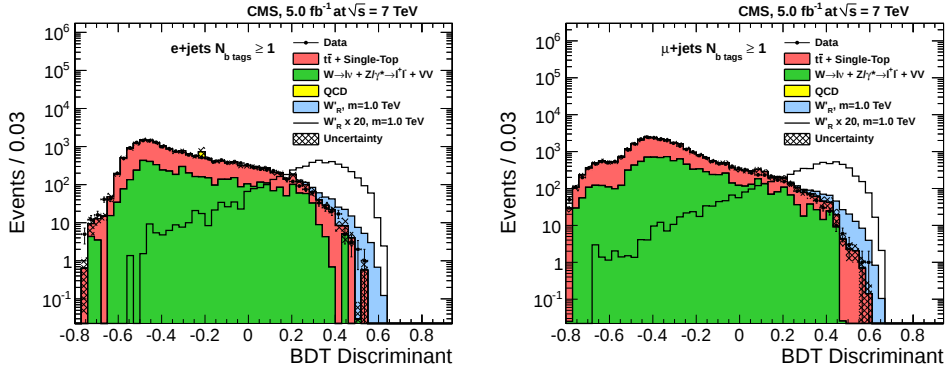
Figure 3: Distribution of the BDT output discriminant. Plots for the e+jets (left) and the \mu +jets (right) samples are shown for data, expected backgrounds, and a W'_R signal with mass of 1 TeV. The hatched bands represent the total normalization uncertainty on the predicted backgrounds.
