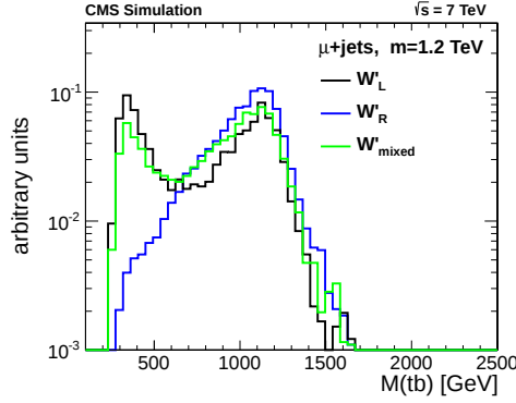
Figure 1: Simulated invariant mass distributions for production of W'_R , W'_L , and W'_{LR} with a mass 1.2 TeV. For the cases of W'_L and W'_{LR} , the invariant mass distributions also include the contribution from s-channel single top quark production and show a minimum corresponding to the destructive interference between the amplitudes for production of left-handed fermions via the W and W'_L bosons. These distributions are after applying the selection criteria described in Sec. 4.
