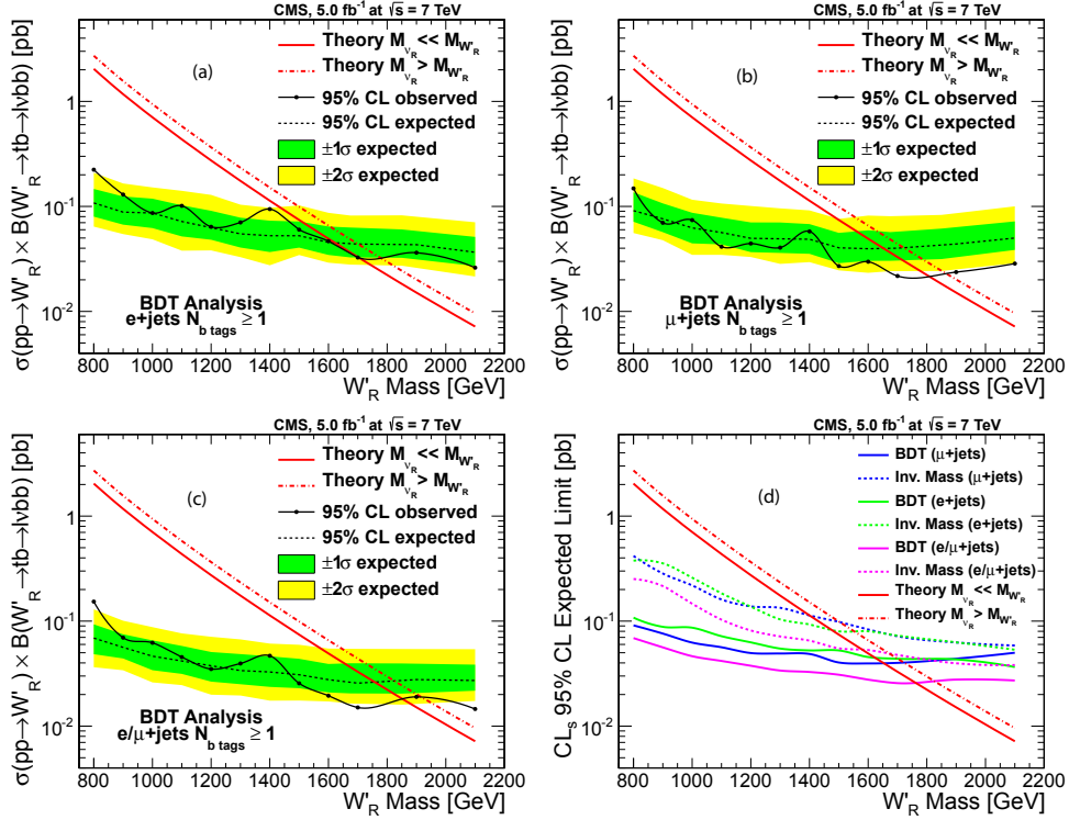
Figure 4: The expected and measured 95% CL upper limits on the production cross section \sigma(pp \rightarrow W')B(W' \rightarrow tb \rightarrow \ell v b b) of right handed W' bosons obtained using the BDT discriminant for \geq 1 b-tagged electron+jets events (a), muon+jets events (b), and combined (c). Also shown (d) is a comparison of the expected 95% CL upper cross section limits obtained using invariant mass distribution and BDT output for right handed W' bosons for \geq 1 b-tagged muon+jet events, electron+jet events, and combined. The \pm 1\sigma and \pm 2\sigma excursions from expected limits are also shown. The solid and dot-dashed red lines represent the theoretical cross section predictions for the two scenarios M_{VR} > M_{W'} , where W' can decay only to quarks and M_{VR} \ll M_{W'} , where all decays of W' are allowed. [16–18].
