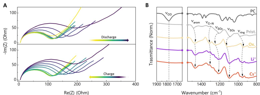
Fig. 4 (A) In situ electrochemical impedance spectroscopy (EIS) collected during the second charge and discharge cycle of the Ca–Zn–PTtSA electrode using 1 mol L −1 KTFPI in propylene carbonate as electrolyte, and at a current density of 10 mA g −1 . One EIS spectrum was recorded after each electrochemical step, consisting of 1 h of charge or discharge followed by a 1 h rest period. (B) Ex situ FTIR spectra of the pristine Ca–Zn–PTtSA (Prist.), electrochemically oxidized □–Zn–PTtSA (Ox.), electrochemically reduced Li 2 –Zn–PTtSA (Li + ), and Cs 2 –Zn–PTtSA (Cs + ) phases, overlaid with the propylene carbonate spectra to highlight characteristic bands.
