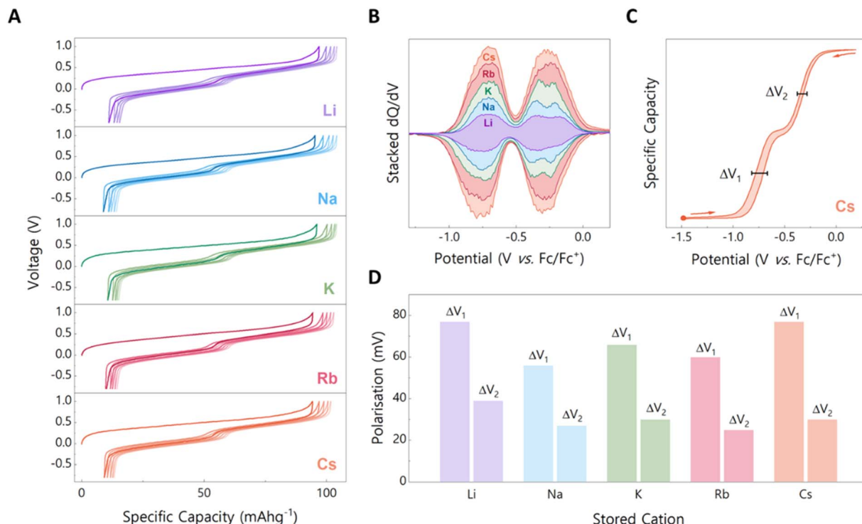
Fig. 2 (A) Galvanostatic charge-discharge profiles over the first five cycles using Ca-Zn-PTtSA as positive electrode material for Li^+ , Na^+ , K^+ , Rb^+ , and Cs^+ storage. Electrolyte used was 1 \text{ mol L}^{-1} MTFSI in propylene carbonate electrolyte; electrodes cycled at current density of 10 \text{ mA g}^{-1} in a three-electrode Ca-Zn-PTtSA||Ag||AC cell. (B) The corresponding dQ/dV plots at cycle 5, stacked on top of each other with a rescaling factor of 2 for visibility. (C) Charge-discharge polarization estimation for Cs^+ storage, as determined at the cycle 5, for a current density of 10 \text{ mA g}^{-1} ; a larger hysteresis is noted for the 1st redox plateau. (D) Comparative analysis of polarization values of the 1st and 2nd plateaus for each 1s-block cation system studied; as determined at the cycle 5, for a current density of 10 \text{ mA g}^{-1} .
