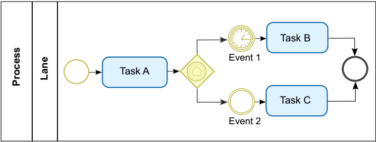
Fig. 4 Implicit decision pattern
