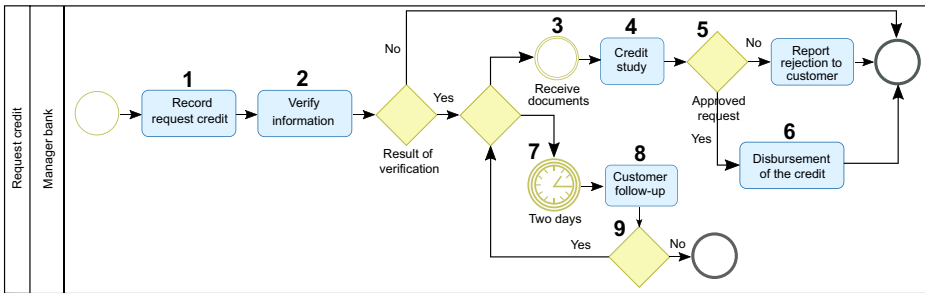
Fig. 10 BPMN model for Problem 2
