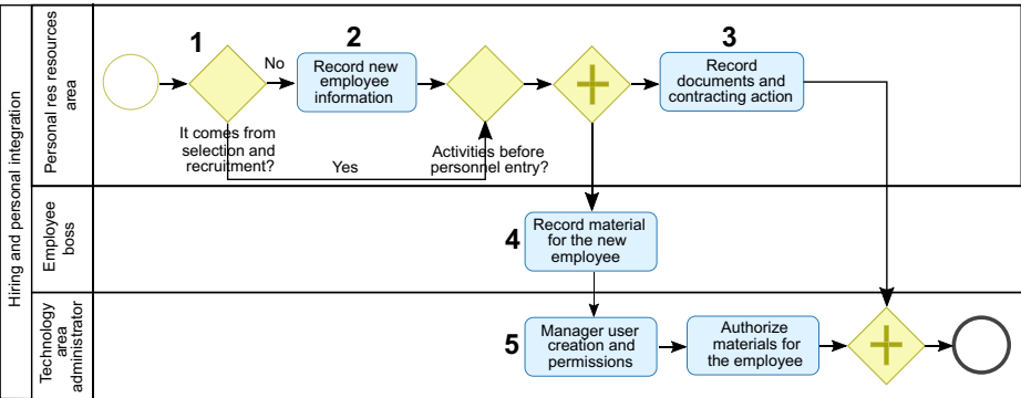
Fig. 8 BPMN model for Problem 1
