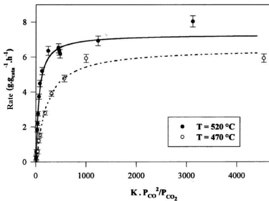
Fig. 2.9. Maximal rates of deposition vs (P_{CO})^2/(P_{CO_2})
