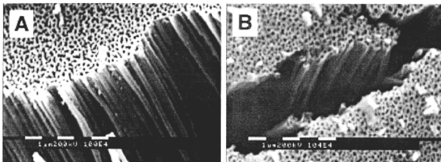
Fig. 2.26. SEM images of CNT obtained by chemical vapor deposition of carbon (CVD, without catalyst) on the walls of pores of an alumina membrane, using ethylene ( A ) and pyrene ( B ), during 10 min at 900°C. The template membranes have been dissolved in concentrated HF [190]. Reproduced with permission from G. Che, B. B. Lakshmi, C. R. Martin, E. R. Fisher, and R. S. Ruoff: Chem. Mater. 10 , 260 (1998), copyright 1998 American Chemical Society
