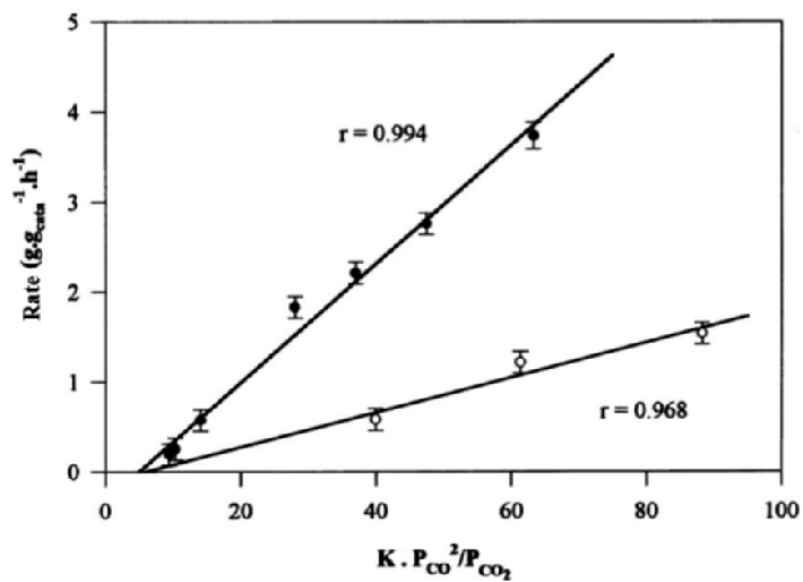
Fig. 2.10. Enlargement of Fig. 2.9 for 'weak' values of (P_{CO})^2/(P_{CO_2})
