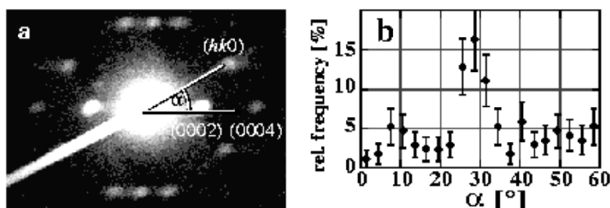
Fig. 2.42. ( Left ) Electron diffraction pattern of a B-doped tube ( Right ) Statistical analysis of the angular distribution of the hk0 reflections. The value \alpha = 30 deg corresponds to the zigzag geometry [255]
