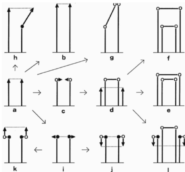
Fig. 2.35. Model for the open-end growth of the nanotube. (Top) The tube ends are open while growing by accumulating carbon atoms at the tube peripheries in the carbon arc. Once the tube is closed, there will be no more growth on that tube but new tube shells start to grow on the side-walls. (Middle) Schematic representation of a kink-site on the tube end periphery. Supplying two carbon atoms (o) to it, the kink advances and thus the tube grows. But the supply of one carbon atom results in a pentagon which transforms the tube to a cone shape. (Bottom) Evolution of carbon nanotube terminations based on the open-end tube growth. Arrows represent passes for the evolution. Arrow heads represents terminations of the tubes and also growth directions. Open and solid circles represents locations of pentagons and heptagons, respectively [225] (see text)
