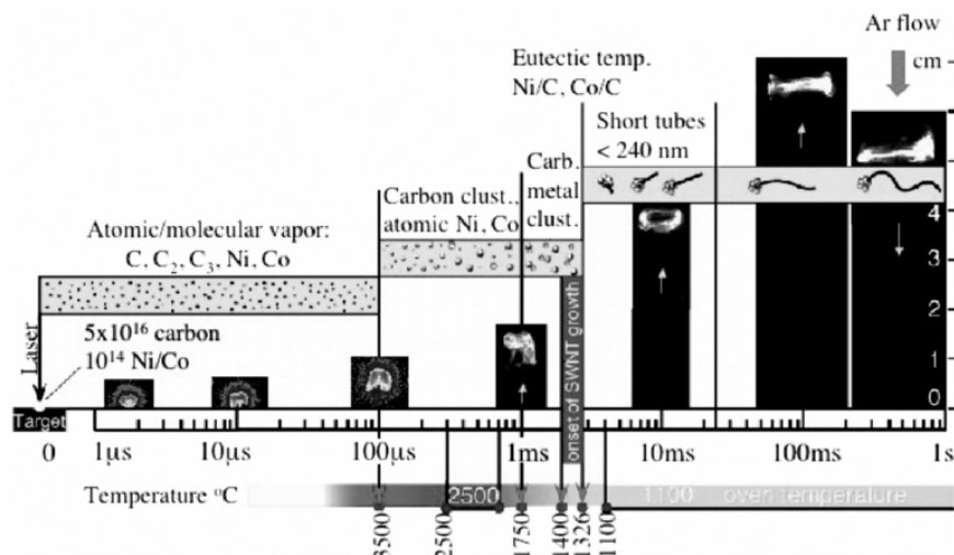
Fig. 2.5. A compendium of the results from Poretzky et al. [41,42], which shows actual images of the ablation plume vs. time (log scale), the species detected spectroscopically from the plasma emission or laser-induced luminescence spectra, plume temperatures measured through blackbody emission above the oven temperature, and lengths measured from arrested-growth experiments
