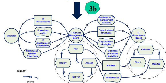
GI-Tropos Strategic Service model
