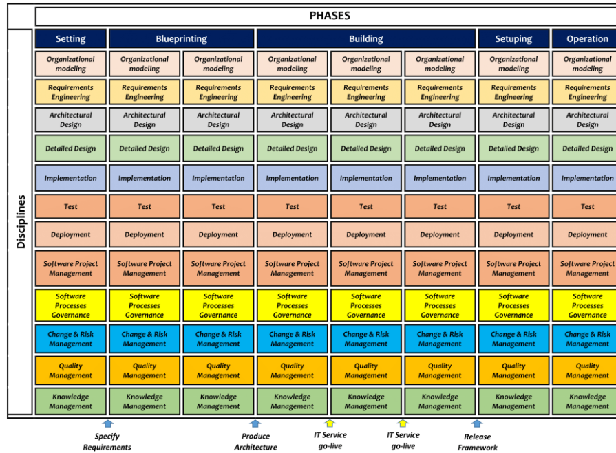
Figure 1: GI-Tropos iterative process framework
