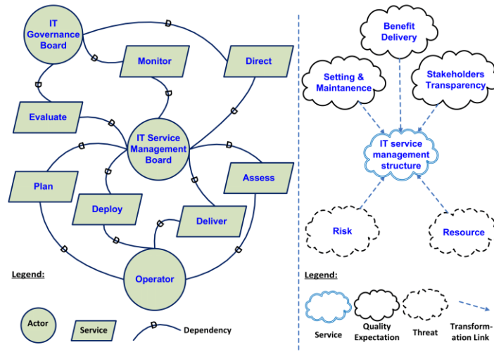
Figure 2-3: GI-Tropos Strategic Service model
