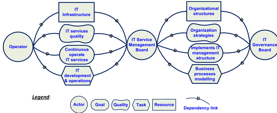
Figure 5: GI-Tropos Strategic Dependency model
