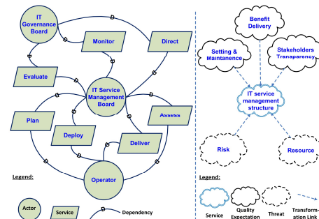
GI-Tropos Strategic Service model
