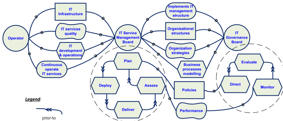
Figure 6: GI-Tropos Strategic Rationale model
