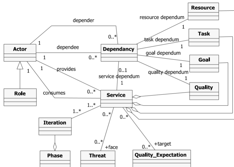
Figure 4: GI-Tropos meta-model
