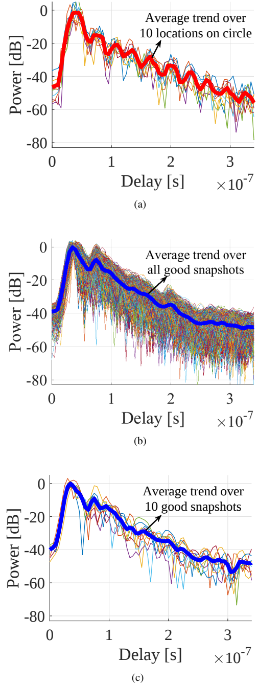
Fig. 8. Numerical example for Rx position No.2: (a) simulated CIR PDP by proposed approach where Rx is on the circle centered at marked position in Fig. 5 (b) measured CIR PDP of each snapshot and the average PDP trend over all good snapshots (c) measured CIR PDP of random 10 good snapshots and the average PDP over these 10 snapshots
