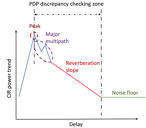
Fig. 7. Demonstration for the PDP trend consisting of peak, major multipaths, reverberation slope and noise floor
