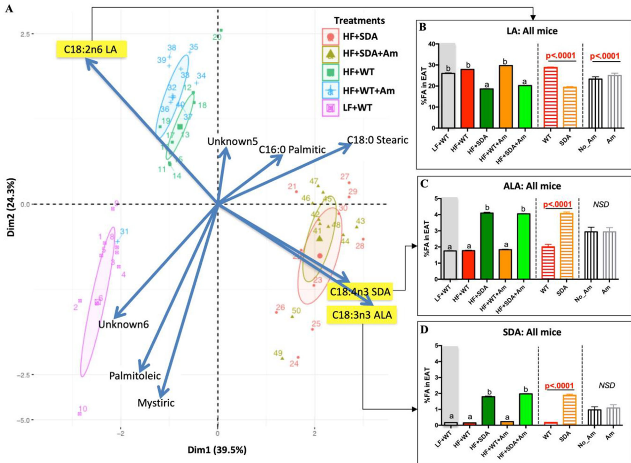
Figure 5. Mice fed an SDA-enriched diet incorporated more n-3 and less n-6 PUFAs into adipose tissue. A) principal component analysis of fatty acid profiles. Arrows are eigenvectors depicting direction towards which a specific fatty acid drives differences among treatments. Ovals represent the 95% confidence interval for data in each treatment. Specific levels of B) linoleic, C) alpha-linolenic, and D) stearidonic acid in epididymal adipose tissue (EAT). Treatments with different letters are significantly different from one another by Tukey Test. Shaded area corresponds to low fat (LF) diet control. Factorial analysis was only performed with high fat (HF) diet-fed treatments by Two-Way ANOVA. p -values from this analysis are presented for main effects and interactions (Oil X Am). Only significant interactions are shown. Significant p -values ( <0.05 ) are shown in red. Marginal p -values ( 0.05 – 0.07 ) are shown in black. NSD means no significant main effects were observed.
