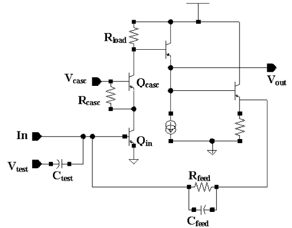
Fig. 2. Current preamplifier.
