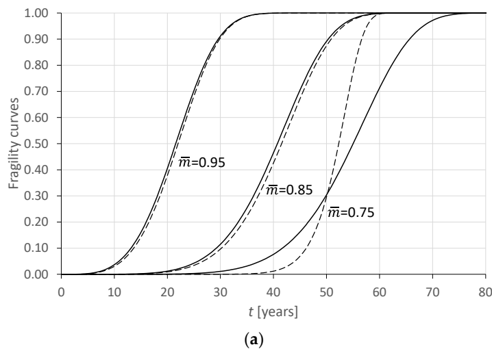
Figure 7. Scenario 1: (a) Comparison between experimental curves obtained for scenario 1 and the fragility curves defined as “statistical truth”. (b) Parameters of the theoretical and experimental distributions compared.
