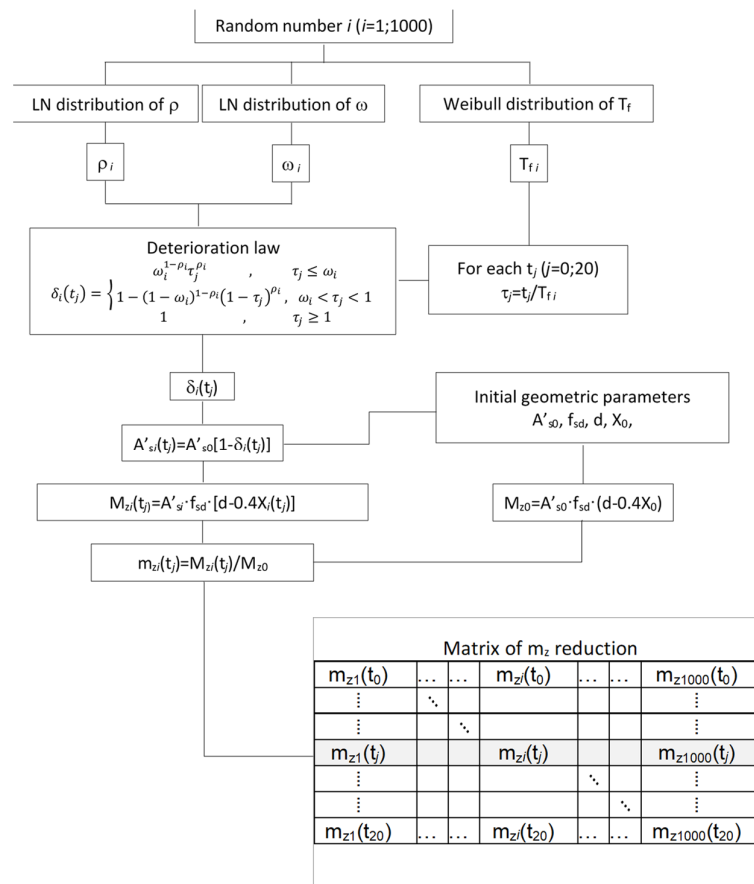
Figure 3. Procedure for probabilistic evaluation of the reduction in resistant action A'_s(t) and the relative decrease in ultimate bending moment m_z(t) . This procedure is repeated 1000 times for 21 different instants of life between 0 and 100 years (with 5-years time step), thus producing 21,000 different samples of potential performance loss.
