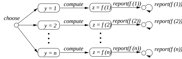
Figure 8: Task-PIOA Trapdoor
