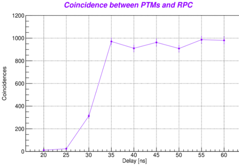
Figure 8.15. | Number of coincidences for different delay values of the RPC signal.
