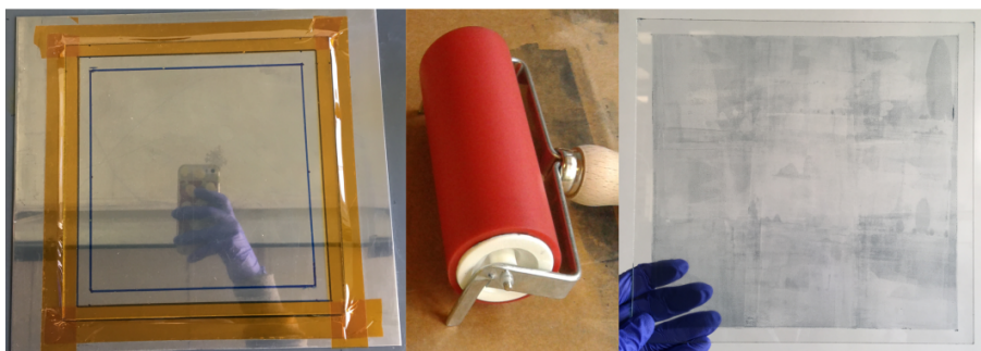
Figure 3.3. | Method to apply the resistive coating on glass plates, (left) Masked glass plate before applying paint, (middle) Roller used to spread paint, (right) Painted a glass plate. Figure from [99].
