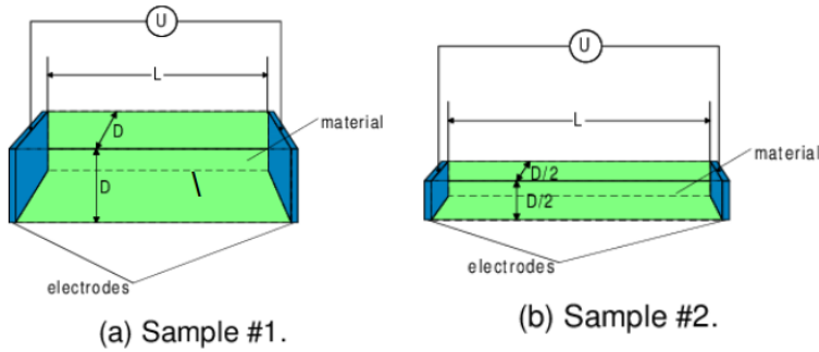
Figure 5.2. | Current density [113].
