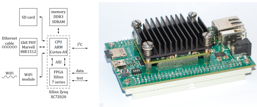
Figure 3.10. | Structure of the FPGA+CPU module [105] (left) Physical view of the module (right).
