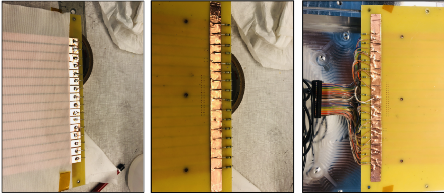
Figure 6.8. | The resistors soldered on signal end and ground end of the strip (Left and center figures, respectively). Readout board with 34 pin connector (right).
