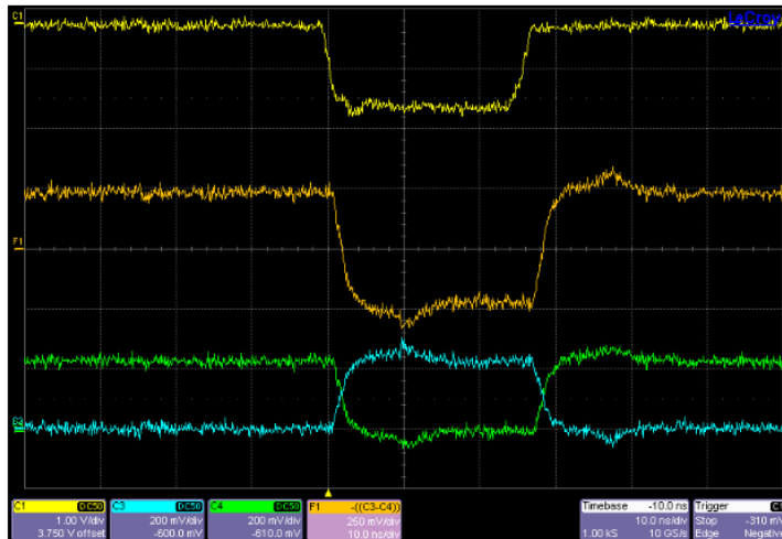
Figure 4.16. | Oscillogram of the LVDS output and monostable output. In the channel 1 (Yellow), it shows the output from monostable and in channels 3 and 4 (blue and green respectively) shows to output from 2 lines of LVDS module.
