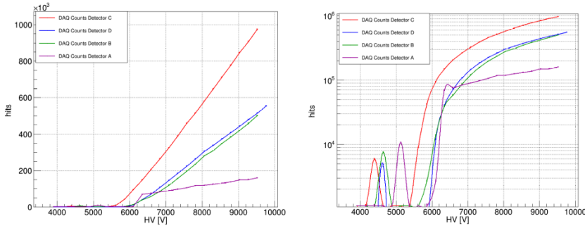
Figure 8.7. | The total hits in each RPC as a function of High voltage supplies. The left figure shows the hits in linear scale and right figure shows the hits in log scale for better understanding of the counts in low voltages.
