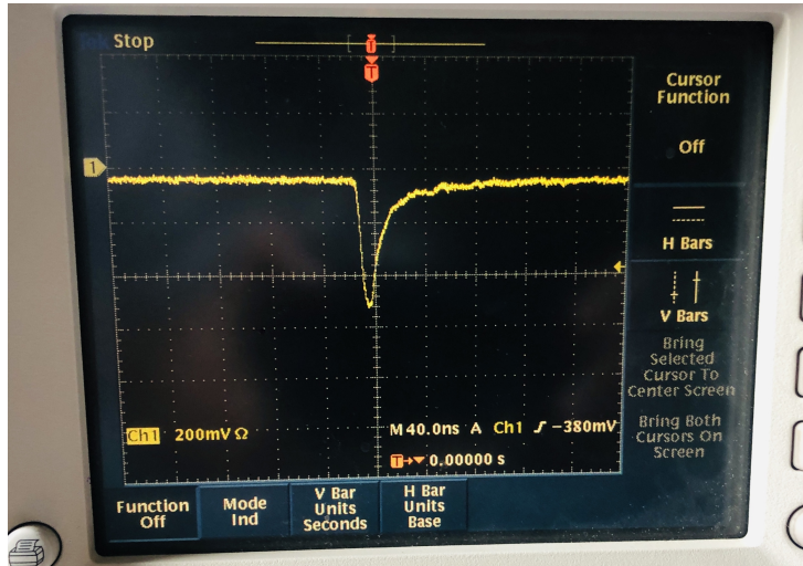
Figure 4.6. | Oscillogram of the scintillator signal of Top(A) PMT . The input impedance of the oscilloscope is 50\Omega , voltage scale is 200 mV/square, and the time scale is 40 ns/square. The trigger of the oscilloscope is set to -380 mV.
