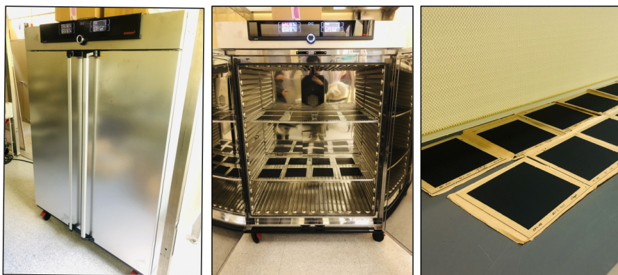
Figure 5.11. | UF750plus lab oven (left). Painted glass plates placed in the oven for curing (middle). The cured plates stored in a white room after measuring the resistivity (right).
