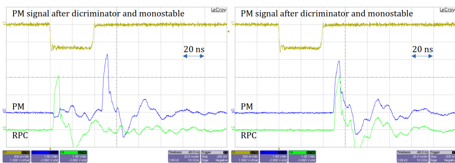
Figure 8.22. | RPC (green) and PMT (blue) signal without any delay (left).RPC (green) signal is delayed with 50 ns and PMT (blue) signal without any delay (right).
