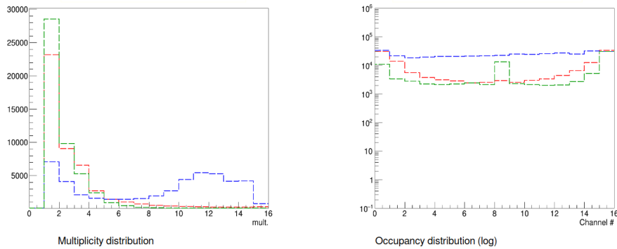
Figure 8.11. | Multiplicity and Occupancy distributions of 3 different RPCs in the CMS clean room. The green plot represents the Readout version 2.1 (See section 6.3), but with 50\Omega termination, the blue plot represents the RPC with readout board version 3.0 (See section 6.4) and red represents the chamber with readout board Version 1.0 (See section 6.4).
