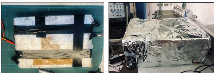
Figure 7.6. | The wrapped RPC with bubble wrap before covering it with Al foil (left) . The cardboard box covered with Al foil after placing RPC inside the box.
