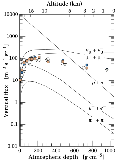
Figure 1.2. | Vertical fluxes of various particles, for momenta larger than 1 \text{ GeV} . Continuous lines are derived from a model and demonstrate that above this energy threshold, at the sea level (maximum atmospheric depth shown in the figure), the sum of positive and negative muon fluxes constitutes the vast majority of the charged particle flux and is only second to the neutrino flux (that is not a background to muography due to the low interaction rate). Points correspond to measurements of the vertical flux of negative muons only, with different. Symbols corresponding to different experiments [8].
