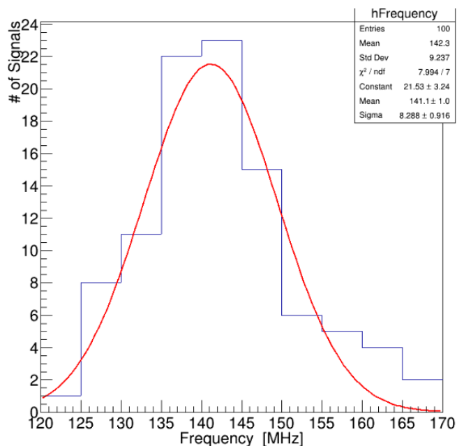
Figure 7.5. | The frequency distribution of the noise, calculated from the signal pattern of the oscilloscope.
