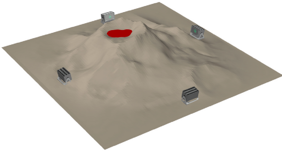
Figure 1.6. | Sketch of muographic measurements aimed at a 3D reconstruction of a volcano (image from [15]).
