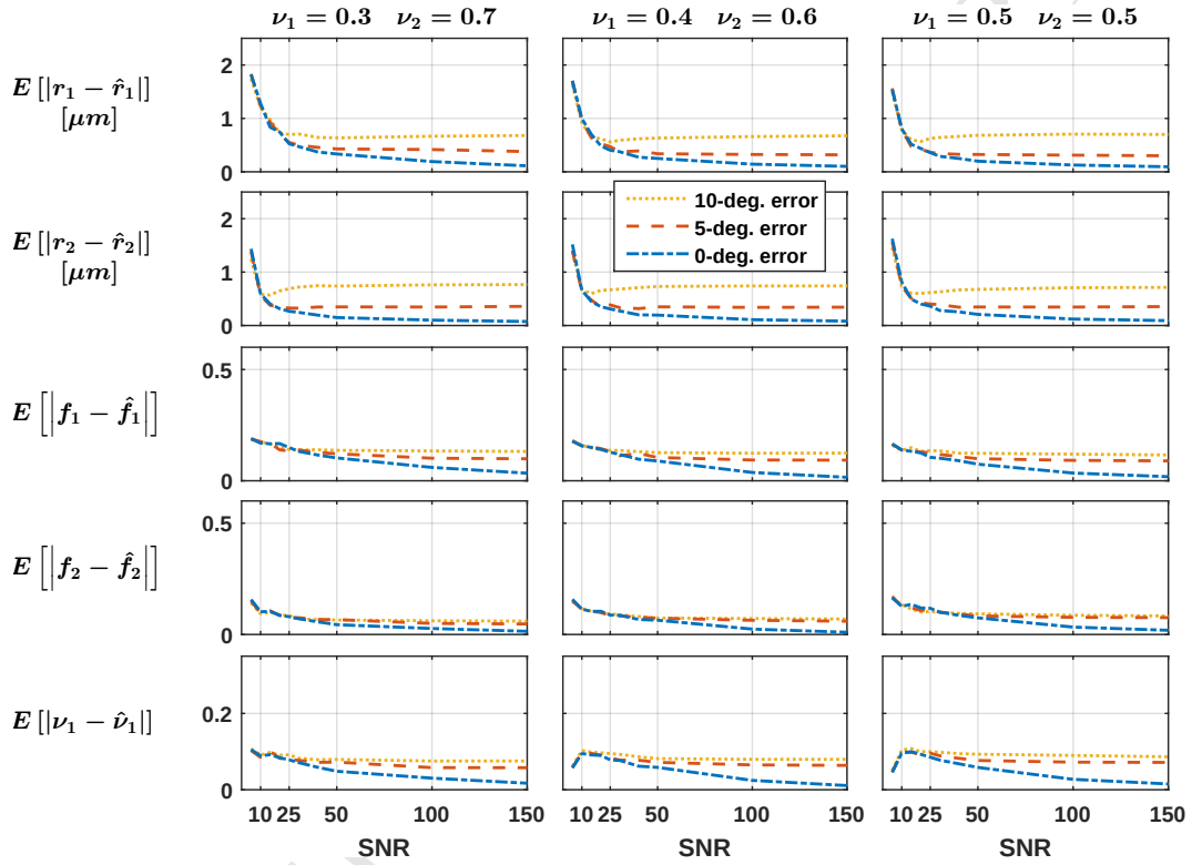
Figure 6: (Exp. 2.A) Errors in the initial estimation of fascicles' orientations yield asymptotically-biased estimates. Mean absolute error on each fascicle's radius index r_1 and r_2 , density index f_1 and f_2 and on the physical volume fraction occupied by the first fascicle \nu_1 . The groundtruth volume fraction of the second fascicle decreases from left to right and the groundtruth crossing angle was fixed to 60^\circ .
