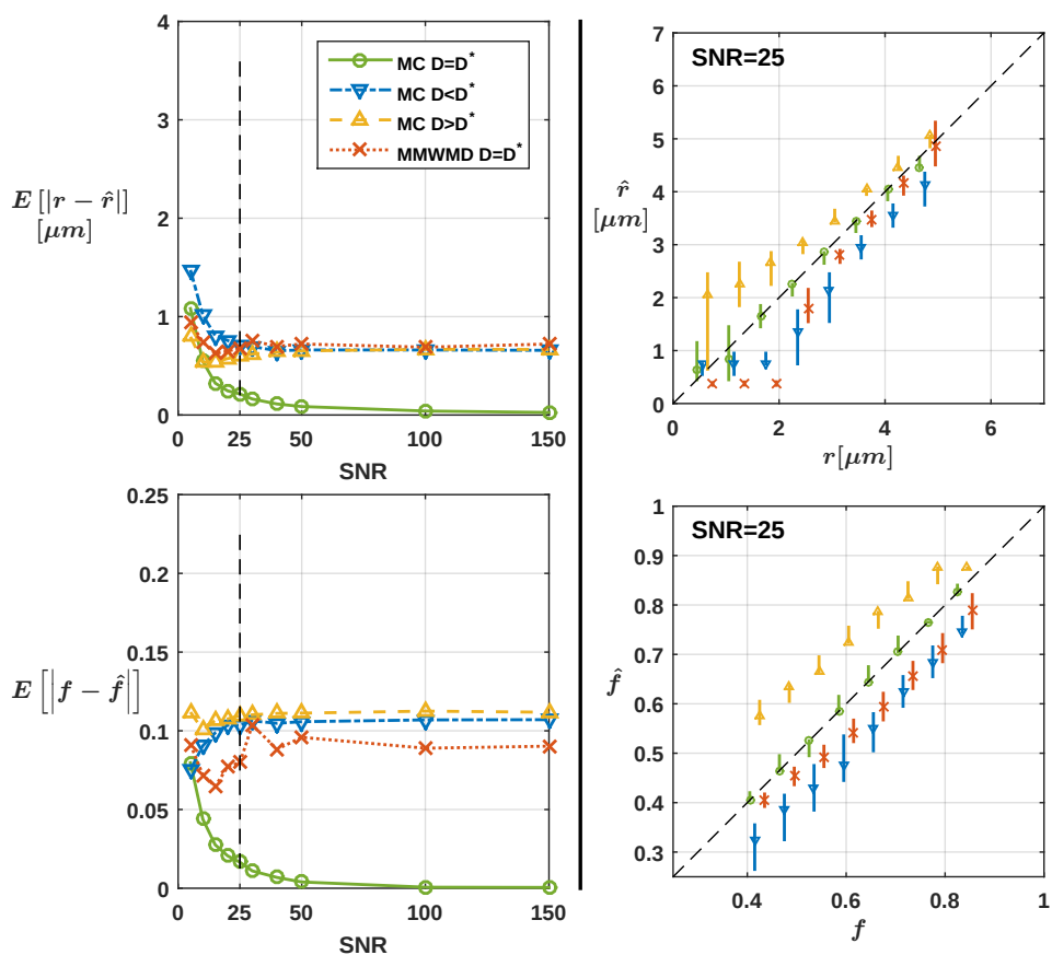
Figure 1: (Exp. 1.A) Consistent microstructural estimates in single fascicles with Monte Carlo (MC) dictionary estimation. The left column displays the mean absolute error on the radius index r (top) and density index f (bottom) as a function of signal-to-noise ratios (SNR). The right column provides a snapshot of estimates at SNR=25, with markers indicating the median over all noise repetitions and groundtruth configurations and bars ranging from the 25th to the 75th percentile of all estimates. Asymptotic errors remained for the minimal model of white matter diffusivity (MMWMD) even though it used the true diffusivity D . 24
