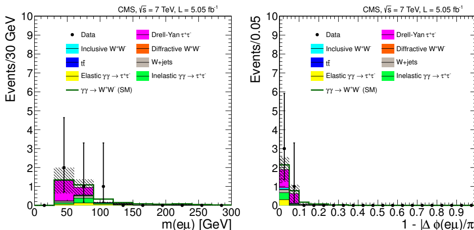
Figure 9. Data compared to simulation for control region 3. The \mu^{\pm}e^{\mp} invariant mass (left) and acoplanarity (right) are displayed for events with zero extra tracks on the \mu^{\pm}e^{\mp} vertex and p_T(\mu^{\pm}e^{\mp}) < 30 GeV. The shaded bands indicate the statistical uncertainty in the background estimation. The signal (open histogram) is shown stacked on top of the backgrounds.
