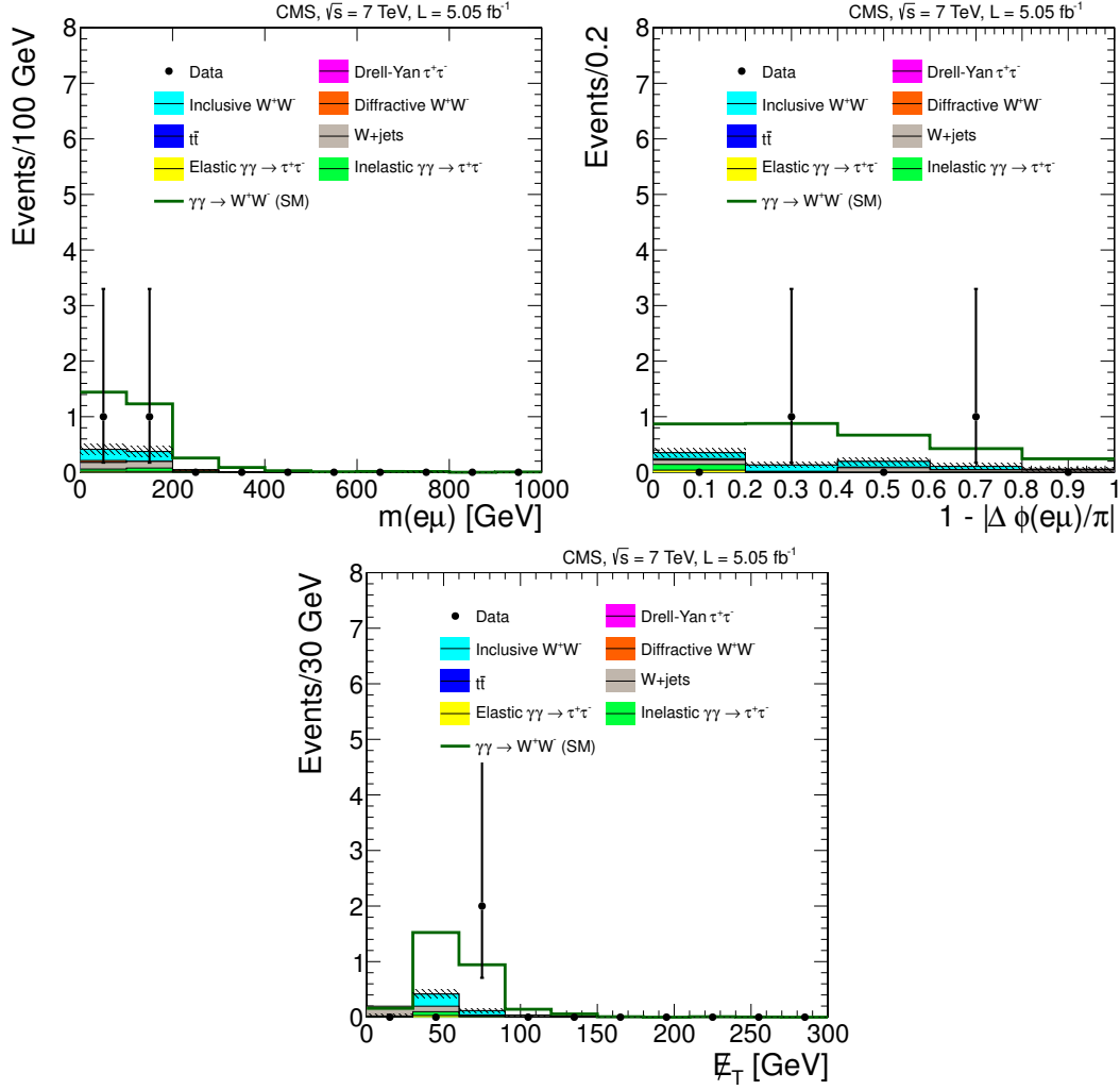
Figure 10. The \mu^\pm e^\mp invariant mass (top left), acoplanarity (top right), and missing transverse energy (bottom) distributions, for events in the signal region with zero extra tracks on the \mu^\pm e^\mp vertex and p_T(\mu^\pm e^\mp) > 30 GeV. The backgrounds (solid histograms) are stacked with statistical uncertainties indicated by the shaded region, the signal (open histogram) is stacked on top of the backgrounds.
