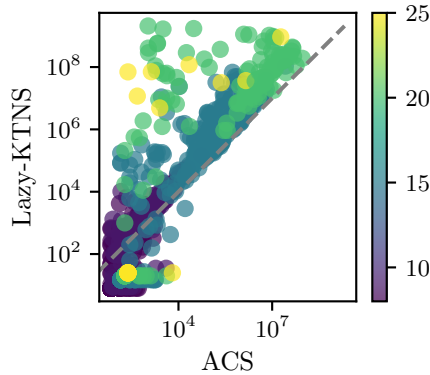
Fig. 7: Comparison of B&B with Lazy-KTNS algorithm and ACS algorithm, regarding the number of explored nodes.
