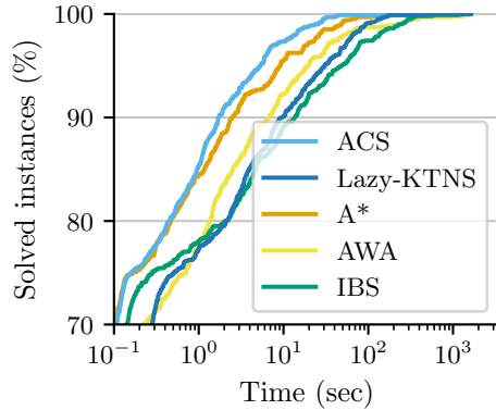
Fig. 5: Percentage of solved instances on dataset A regarding the time (in seconds) with n = \{8, 9, 15\} .
