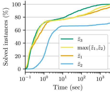
Fig. 3: Percentage of solved instances on dataset A regarding the time (in seconds) with n = \{8, 9, 15\} for all lower bound defined in Section 2.1.
