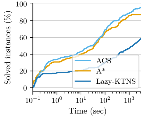
Fig. 6: Percentage of solved instances on dataset A regarding the time (in seconds) with n = \{20, 25\} .
