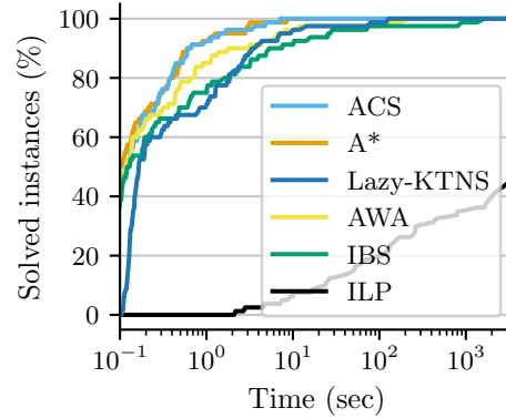
Fig. 8: Percentage of solved instances on dataset B regarding the time (in seconds) with n = \{10, 15\} .
