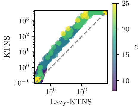
Fig. 4: Comparison of B&B with Lazy-KTNS algorithm and the B&B with KTNS algorithm, regarding the time to find the optimum solution and prove it. Each dot represents an instance of the dataset A.
