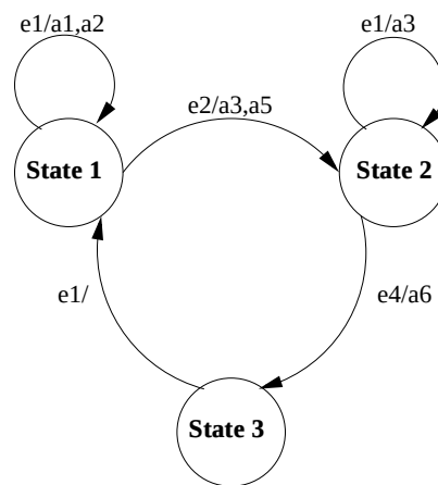
Figure 2-10 State-transition diagram specifying UI events and actions.
