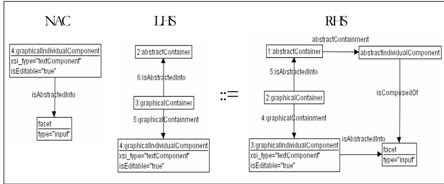
Rule 4-16 Creation of a facet at the abstract level derived from a type analysis of graphical individual components
