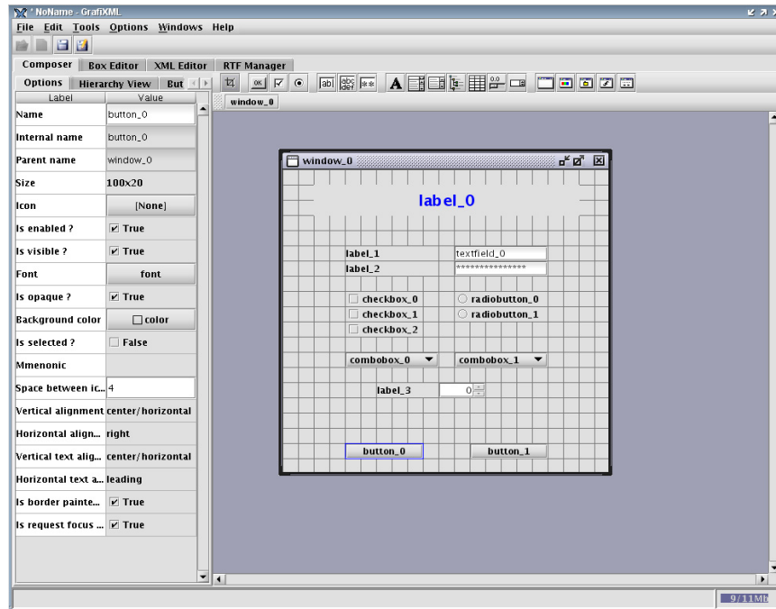
Figure A-4 GrafiXML main window
