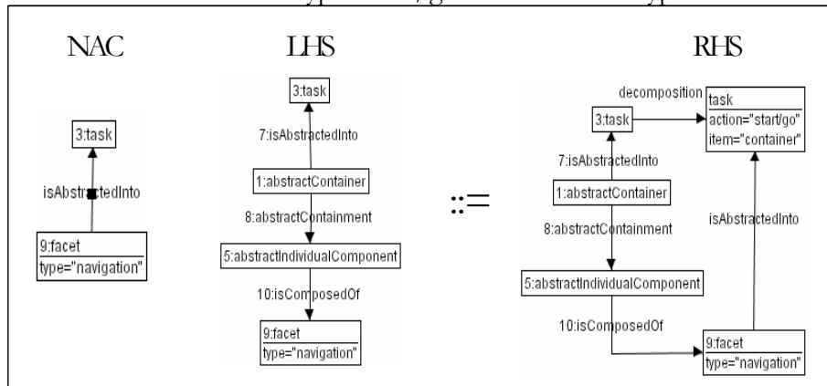
Rule 4-17 Definition of task action types derived from an analysis of facets at the abstract level
