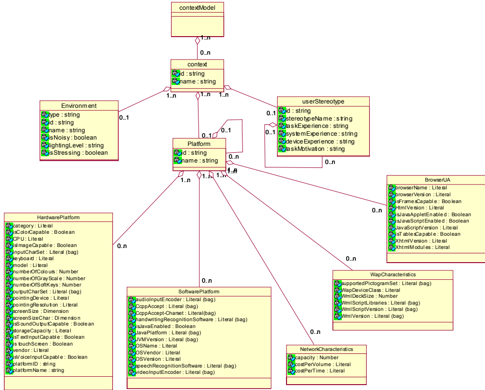
Figure 3-15 Context model
