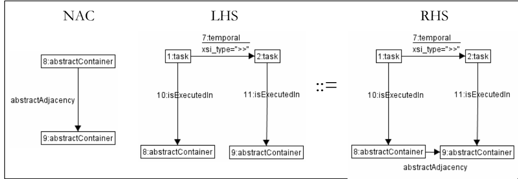
Rule 5-13 Deriving abstract adjacency for <AC,AC> couple
