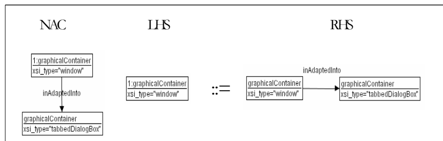
Rule 4-22 Initializing of the adaptation process by creating graphical component to adapt into
