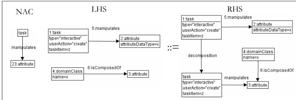
Rule 5-27 Creating sub-tasks for tasks manipulating complex types
