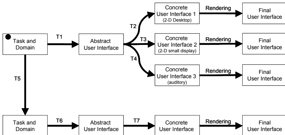
Figure 5-15 Development scenario for case study 2
