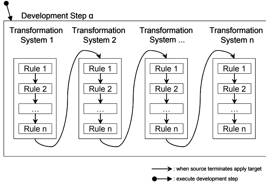
Figure 4-16 An ordered application strategy
