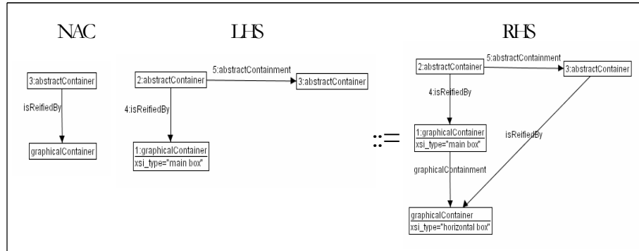
Rule 4-10 A generation of window structure derived from containment relationship at the abstract level
