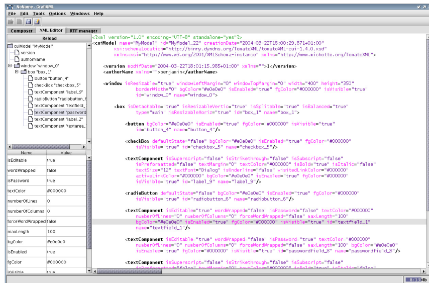
Figure A-5 UsiXML textual editor within GrafiXML tool
