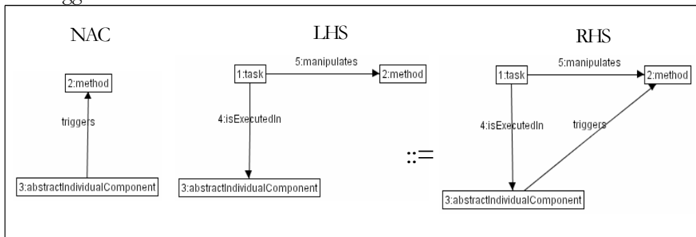
Rule 4-6 Deriving triggering relationships from task domain mappings
