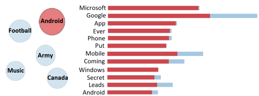
Figure 1. LDA illustration. Exemplary clusters are on the left. Associated words are on the right, with the ratio between their number of appearances in the cluster (in red) and their number of appearances in all clusters (in blue).
