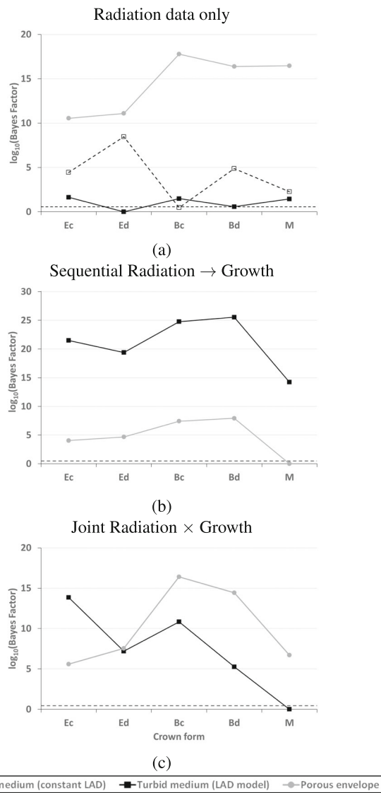
Fig. 3 Bayes factors of the models fitted for each crown form and each considered option according to (a) the “Radiation data only,” (b) the “Sequential Radiation → Growth” and (c) the “Joint Radiation × Growth” optimization schemes. For each “crown form × model configuration × optimization scheme” combination, the Bayes factor is determined as the ratio between the highest marginal likelihood value observed among all model fits carried out for the corresponding optimization scheme and the marginal likelihood value of the model fit for the given combination. The Bayes factors are presented in logarithmic scale for legibility of the figures. The dashed horizontal lines indicate the value 0.5, corresponding to the threshold above which substantial evidence appears in favor of the model fit with the highest marginal likelihood value (i.e., the model fit for which \log_{10}(BF) = 0 )
