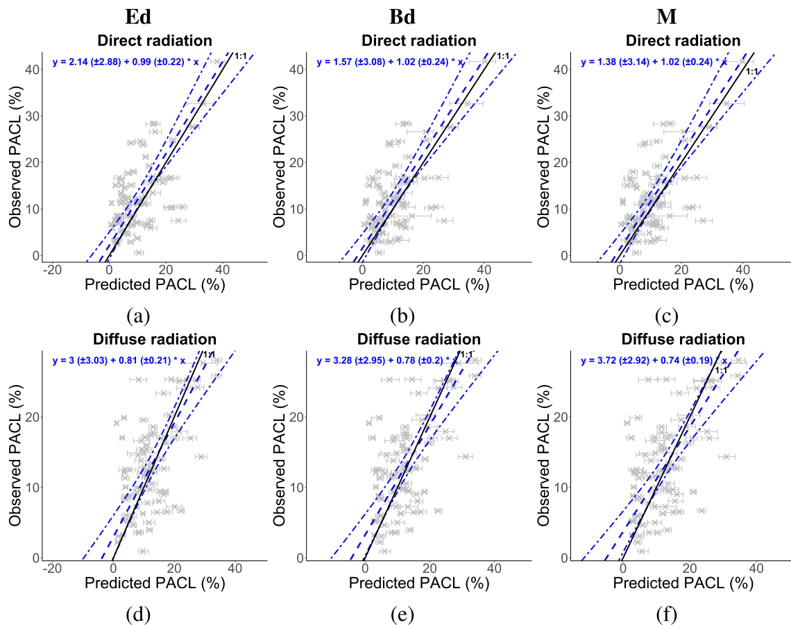
Fig. 4 Comparison of observed and predicted percentages of above canopy light ( PACL ) for (a, b, c) direct and (d, e, f) diffuse radiation considering the “ Radiation data only ” optimization strategy for the “Ed,” “Bd” and “M” crown forms, using the turbid medium radiative transfer formulation. The star symbols represent individual observed PACL values for each considered measurement location as a function of corresponding median values for the distributions of PACL
