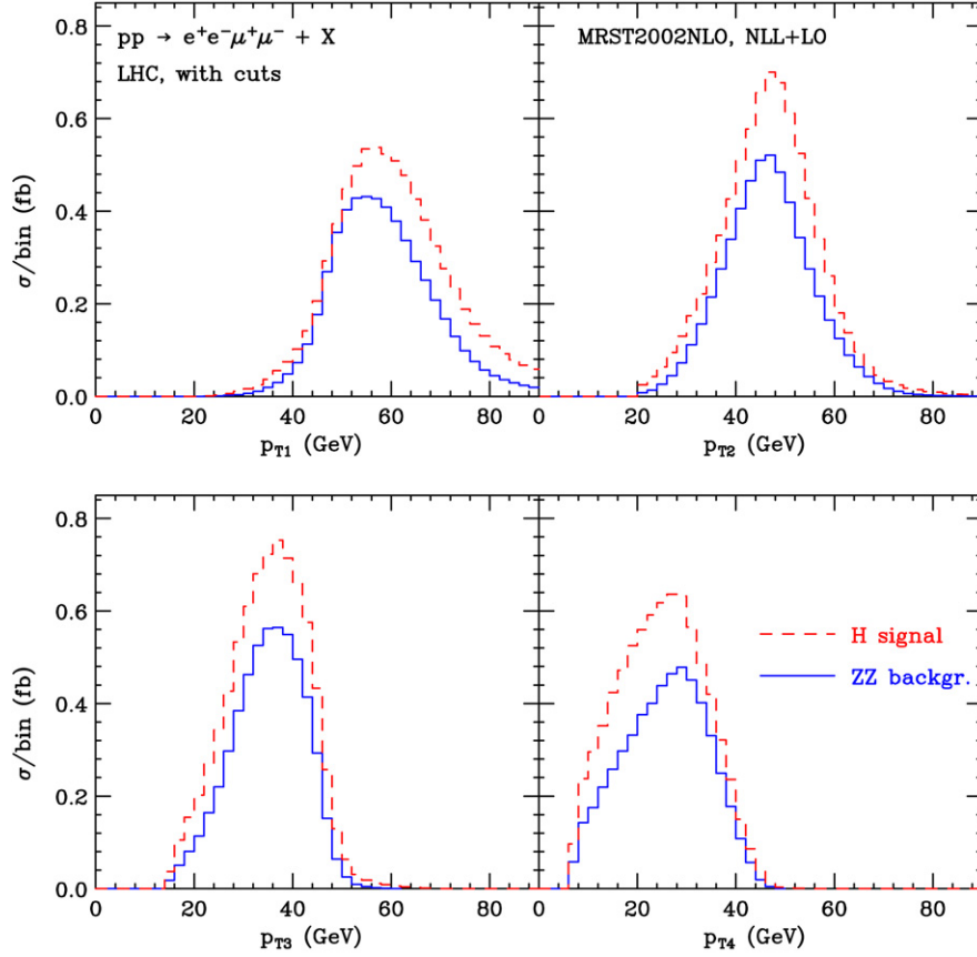
Fig. 6. Leptons p_T spectra for Higgs signal (dashes) and ZZ background (solid).
