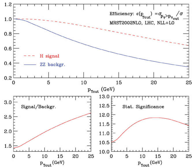
Fig. 9. The upper plot shows the NLL + LO efficiency as a function of p_{T\text{cut}} for the Higgs signal (dashed) and the ZZ background (solid). The lower left plot shows the signal over background ratio and the lower right the statistical significance for an integrated luminosity of 10 \text{ fb}^{-1} .
