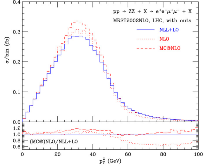
Fig. 3. Comparison of the transverse momentum spectra of one of the Z at NLL + LO (solid) with NLO (dots) and MC@NLO (dashed) results. The lower part of the plot shows the NLO and MC@NLO results normalized to NLL + LO.
