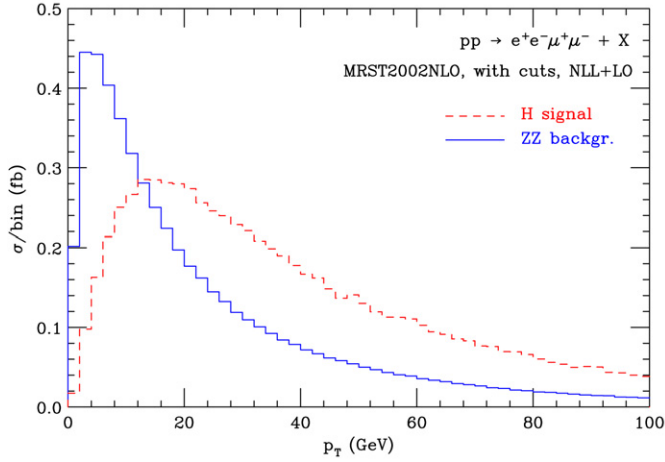
Fig. 8. Comparison of p_T spectra of signal and background at NLL + LO, when standard cuts are applied.
