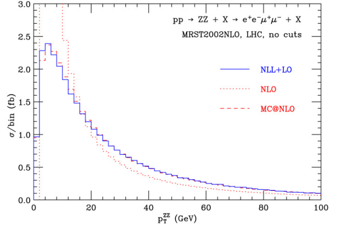
Fig. 1. Comparison of the transverse momentum spectra of the ZZ pair obtained at NLL + LO (solid) with MC@NLO (dashes) and NLO results (dots). No cuts are applied.
