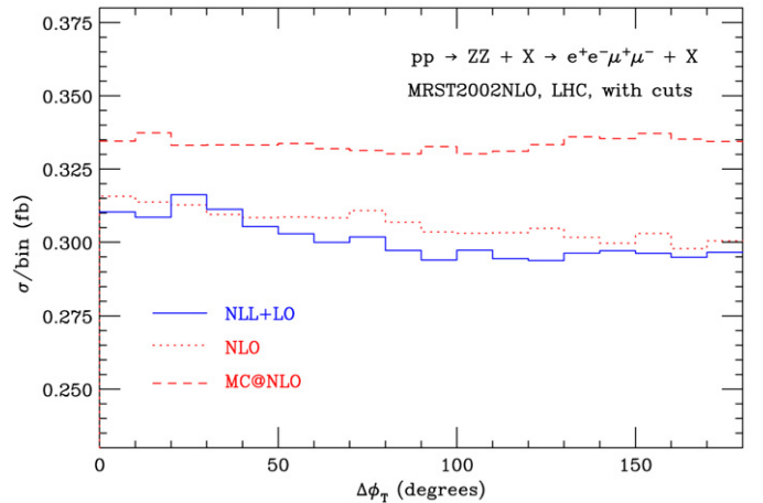
Fig. 5. Same as in Fig. 4 but for the \Delta\phi_T distribution.
