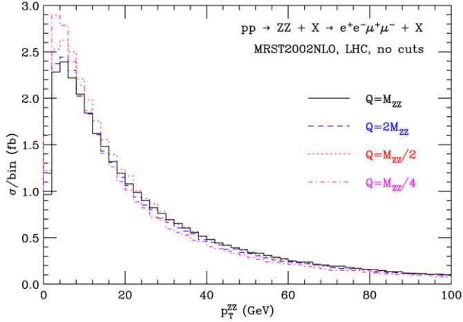
Fig. 2. Comparison of the transverse momentum spectra of the ZZ pair obtained at NLL + LO for different values of the resummation scale Q . No cuts are applied.
