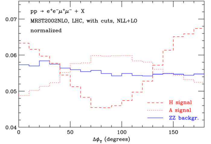
Fig. 7. The \Delta\phi_T distribution for scalar (dashes), pseudo-scalar (dots) and ZZ background (solid) at NLL + LO.
