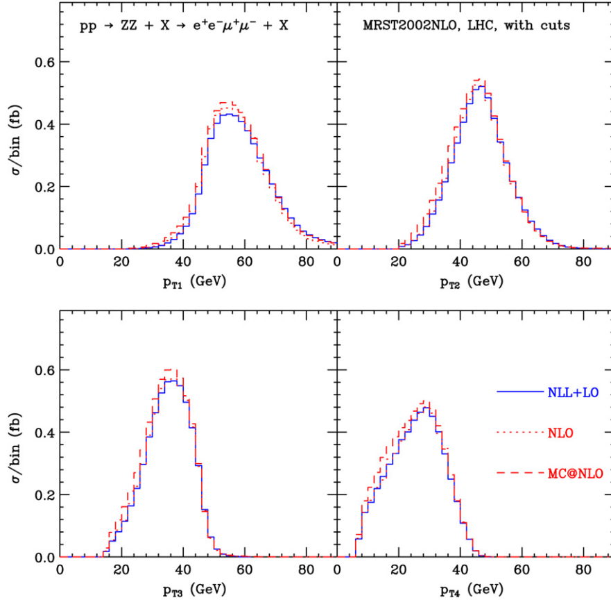
Fig. 4. Transverse momentum spectra of the leptons: NLL + LO (solid), MC@NLO (dashes) and NLO (dots).
