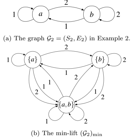
Fig. 2. Example of a min-lifted graph
