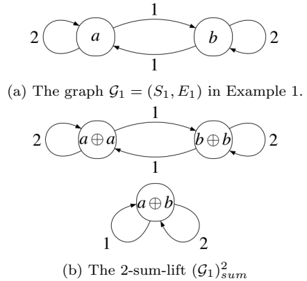
Fig. 1. Example of a 2-sum-lifted graph
