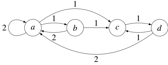
(a) The graph \mathcal{G}_3 = (S_3, E_3) in Example 3
