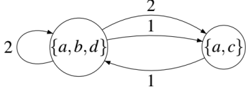
(b) \mathcal{G}_4 = (S_4, E_4) , the strongly connected and path-complete component of (\mathcal{G}_3)_{\min} considered in Example 3
