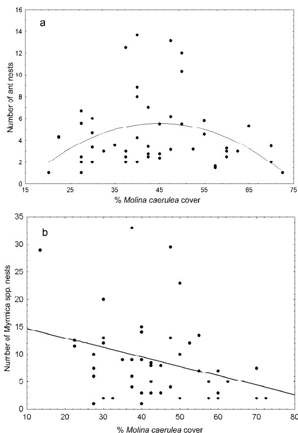
Fig. 2. a – number of ants nests as a function of percent Molinia caerulea cover. The line is a fit of a polynomial regression of the second order; b – number of Myrmica ant nests as a function of percent Molinia caerulea cover. The line is a fit of a simple regression.
