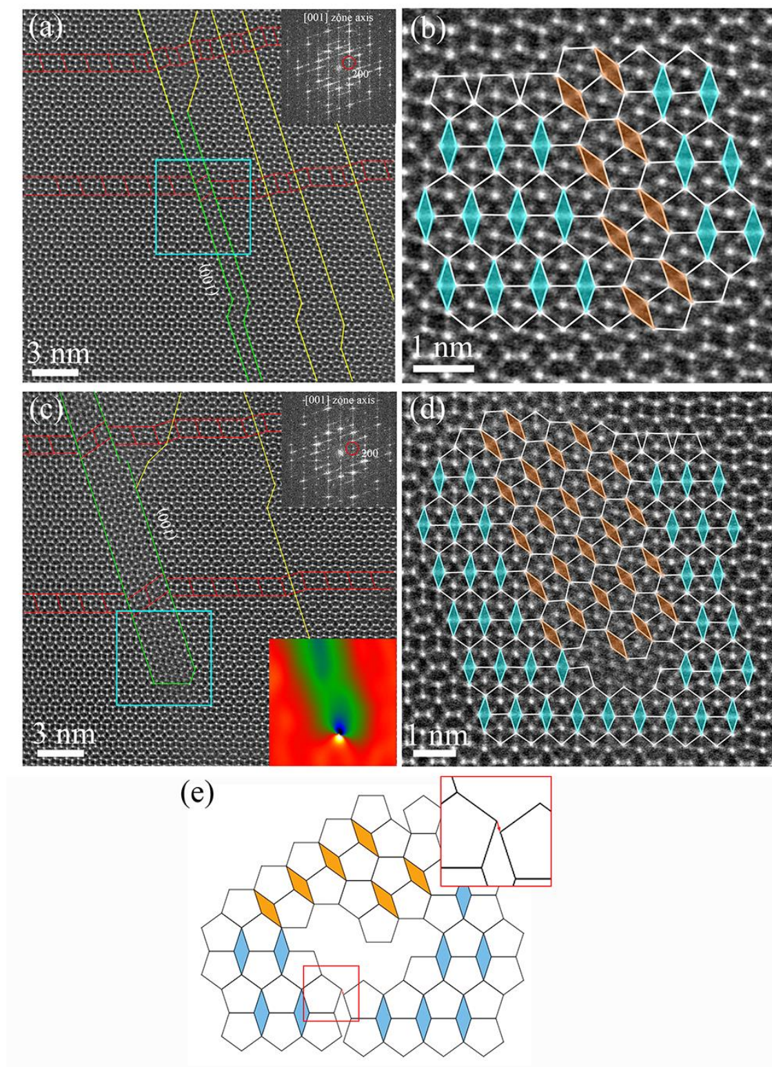
Fig. 4. (a and c) HAADF-STEM images of two planar defects with larger thickness (marked by green lines). (b and d) are enlarged HAADF-STEM images corresponding to the blue squares in (a) and (c), respectively. Stacking faults and twins are marked by green lines in (a) and (c) while APBs are indicated by yellow lines. The change of pentagon/rhomb tilting at stacking fault and twins are superimposed and highlighted in orange. Local g map of
