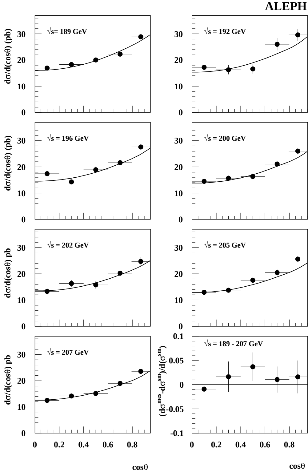
Figure 5: Measured differential cross sections for q\bar{q} exclusive production (closed symbols), as a function of polar angle and for several centre-of-mass energies. The full curves indicate the ZFITTER predictions. The right bottom plot shows the luminosity weighted sum of the differences between the measurements and the Standard Model predictions, normalized to the luminosity weighted sum of the predicted cross sections, for all energy points together.
