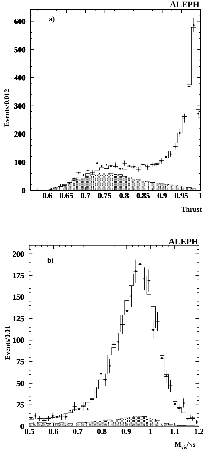
Figure 2: For exclusive hadronic final states, at \sqrt{s} = 207 \text{ GeV} , the distributions of the event thrust (a) and of the visible mass (normalized to the collision energy) for events with thrust > 0.85 (b). The data (dots) are compared to the Monte Carlo expectation (histograms). The shaded areas show the background contribution.
