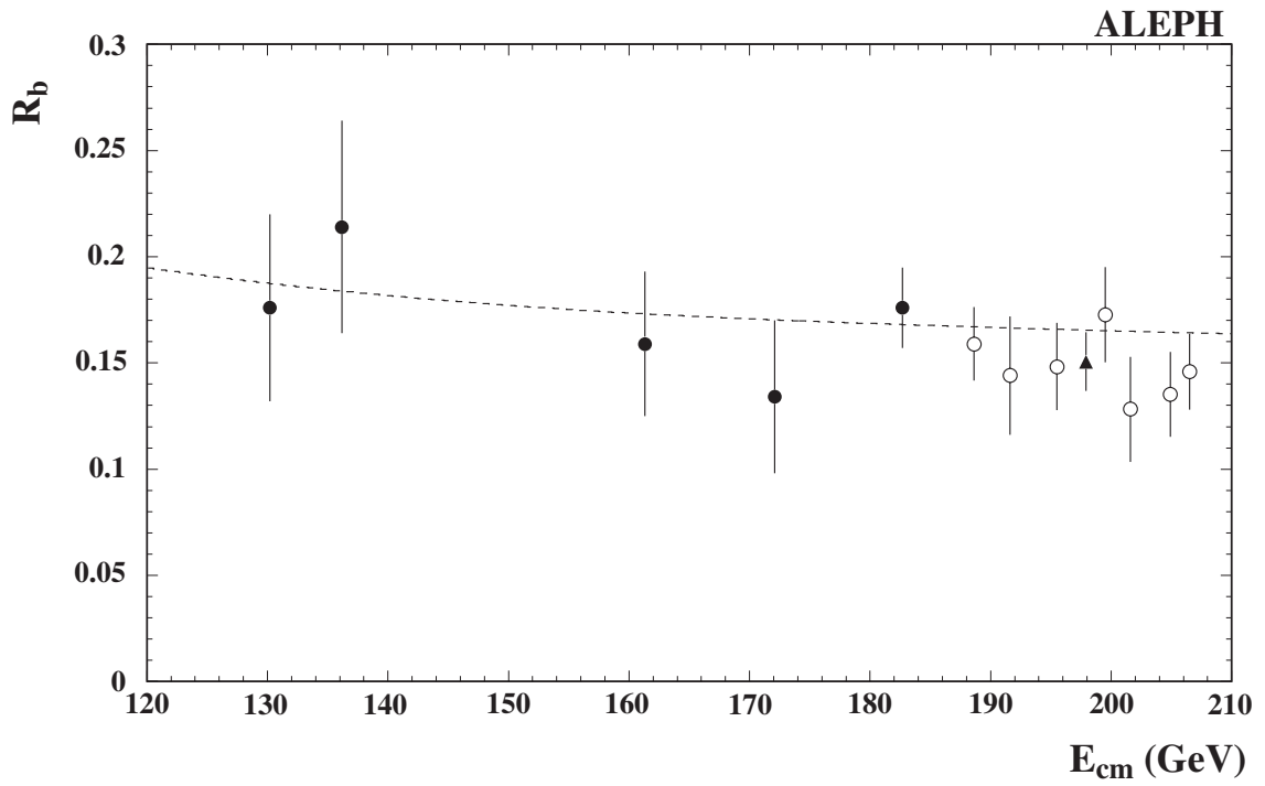
Figure 16: Measured values of R_b (open symbols), as a function of centre-of-mass energy, together with the SM prediction (dashed curve). The dots show previous results [1] and the triangle the average value obtained over the 189-209 GeV energy range.
