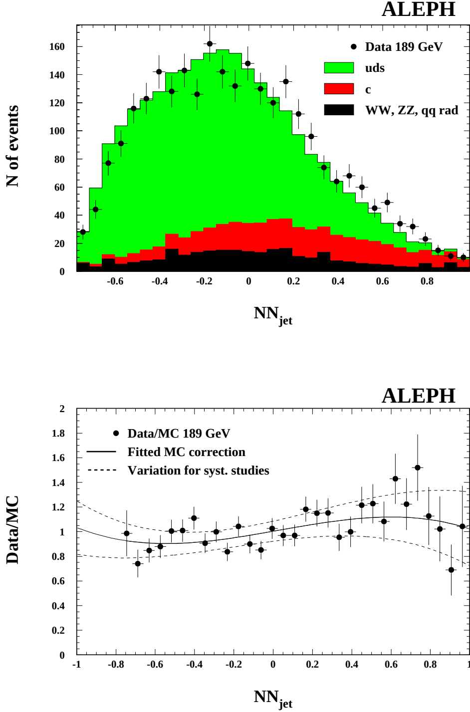
Figure 17: Top: output of the c -tag Neural Network for a uds -enriched sample from the data (dots) and the simulation (histograms). The Monte Carlo distribution is normalized to the data. Bottom: ratio between data and Monte Carlo as a function of the Neural Network output for a uds -enriched sample. The third degree polynomial fit to this distribution (full curve with the error band) is used to correct the simulation (see text).
