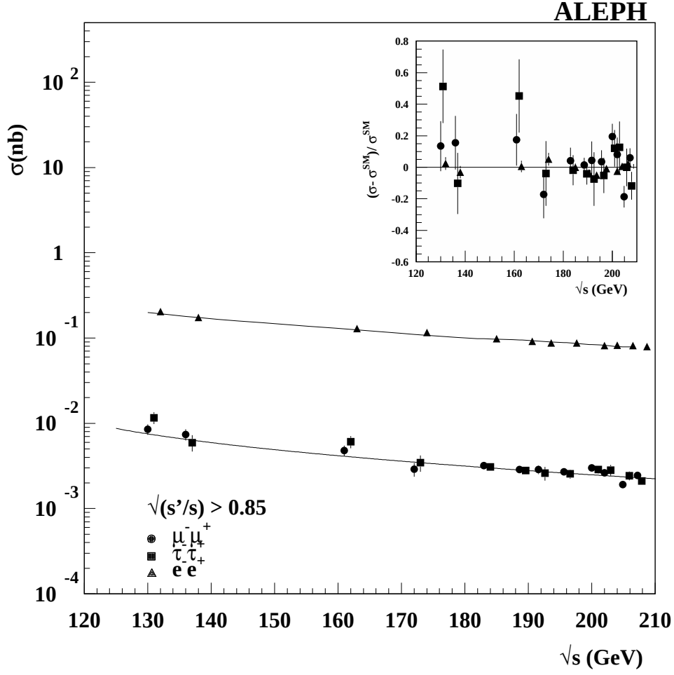
Figure 8: Measured exclusive cross sections for di-lepton production ( |\cos \theta^*| < 0.9 range for the e^+e^- channel), as a function of the centre-of-mass energy (points are shifted for visibility). The full curves indicate the BHWIDE prediction for the e^+e^- channel and the ZFITTER prediction for the \mu^+\mu^- channel. The insert shows the difference between the measurements and the Standard Model predictions, normalized to the predicted cross sections. Measurements at centre-of-mass energies below 189 GeV are from Ref. [1], corrected for the different definition of the exclusive processes.
