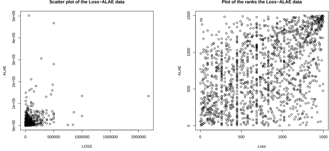
Figure 4: The insurance claims Loss-ALAE data.
