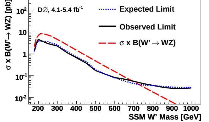
FIG. 3: (color online) The excluded production cross section for an SSM W' boson as a function of the W' boson mass. The excluded mass region is the region where the SSM W' cross section exceeds the excluded cross section.
