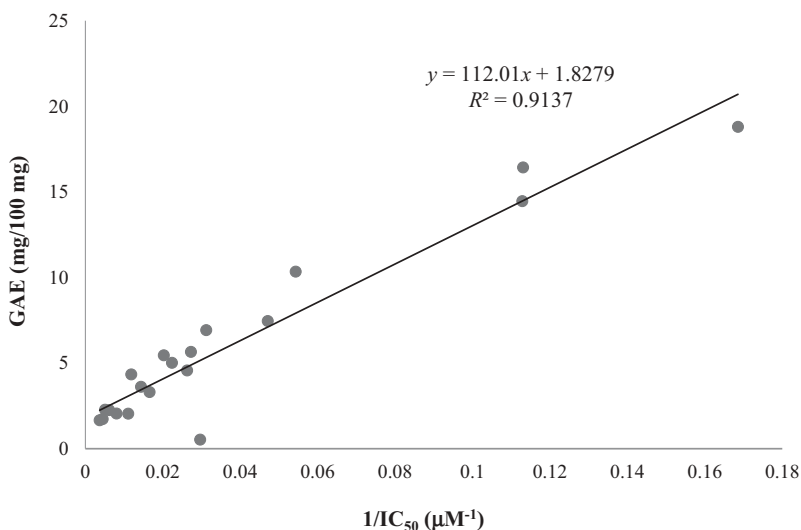
Figure 1. Correlation between phenolic compounds contents (expressed as mg GAE/100 mg extract) and antioxidant activity measured in the DPPH assay (expressed as 1/IC_{50} , \mu M -1 ) of the 23 selected extracts.
