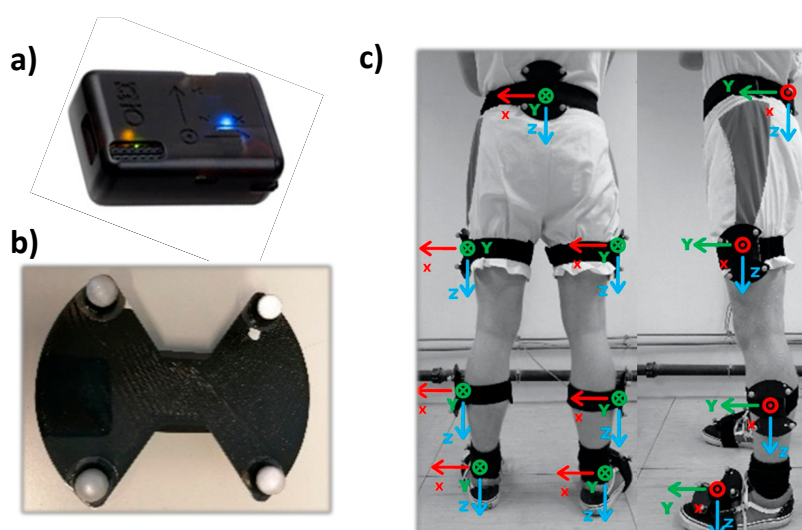
Figure 1. Sensor locations: (a) x-IMU from xi-o Technologies, (b) 3D-printed acrylonitrile butadiene styrene (ABS) enclosures (4 markers of 14 mm diameter) with the inertial measurement unit (IMU) reference frame, and (c) segment reference frame of the 7 IMUs on the subject.
