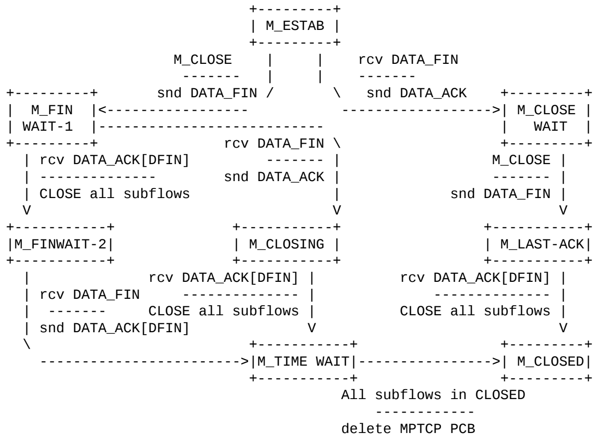
Figure 17: Finite State Machine for Connection Closure
