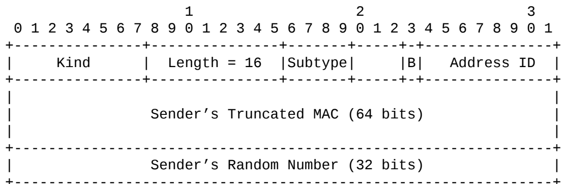
Figure 6: Join Connection (MP_JOIN) option (for responding SYN/ACK)
