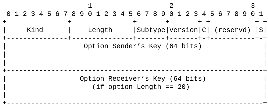
Figure 4: Multipath Capable (MP_CAPABLE) option
