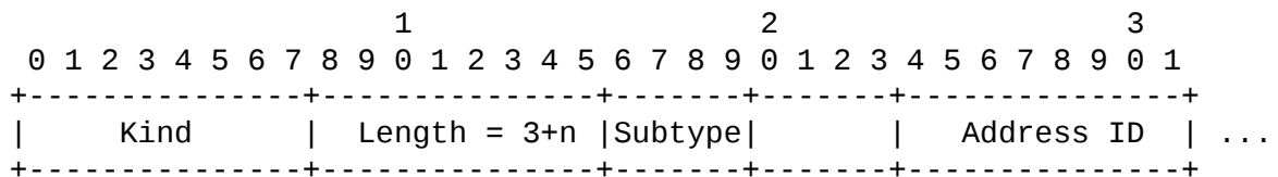
Figure 13: Remove Address (REMOVE_ADDR) option
