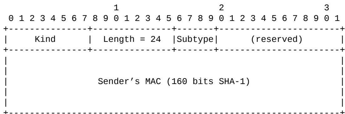
Figure 7: Join Connection (MP_JOIN) option (for third ACK)
