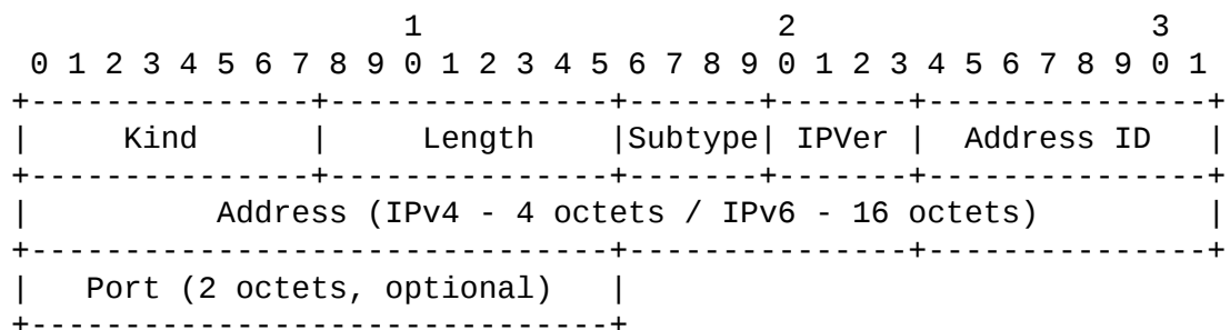
Figure 12: Add Address (ADD_ADDR) option (shown for IPv4)
