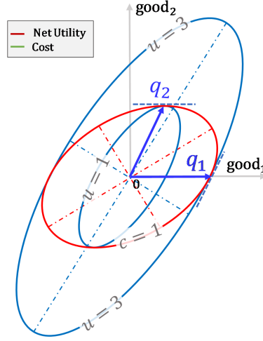
Figure 8: Matrices C and D are simultaneously diagonalized by a pair of bundles (q_1, q_2) that are conjugate diameters in the iso-cost ellipse \frac{1}{2}q^\top Cq and the iso-net-utility ellipse \frac{1}{2}q^\top D^{-1}q . Data examples in Appendix B.1 are used in this figure.
