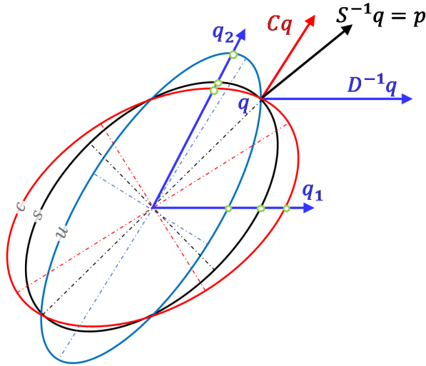
Figure 9: The iso-net utility (blue), iso-cost (red) and the iso-reported-cost (black) ellipses for a production level q . The three ellipses have a pair of conjugate diameters in common which are proportional to q_1 and q_2 .
