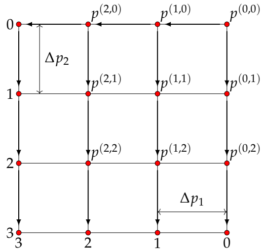
Figure 10: Price grid for numerical integration of \mathbf{s}^{\text{PDE}}(\mathbf{p}) .
