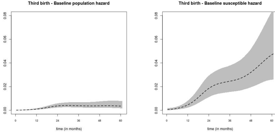
Figure 6: third birth - Fitted baseline population hazard (left) and fitted baseline hazard for susceptible women (right) with 95% pointwise credible intervals.
