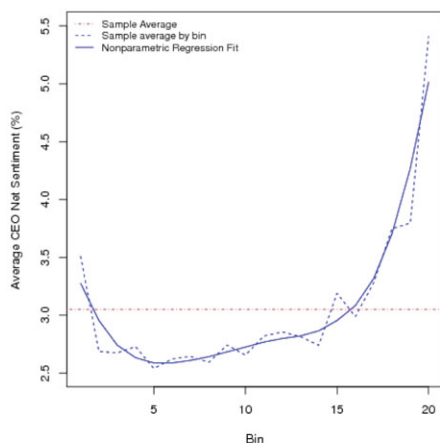
(a) Frequency plot of average positive sentiment by bin (DICTION)—A U-shape and smile in positive sentiment
