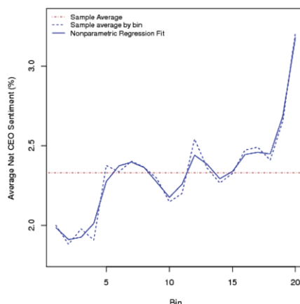
(c) Frequency plot of average net sentiment by bin—A right-sided smirk in net sentiment
