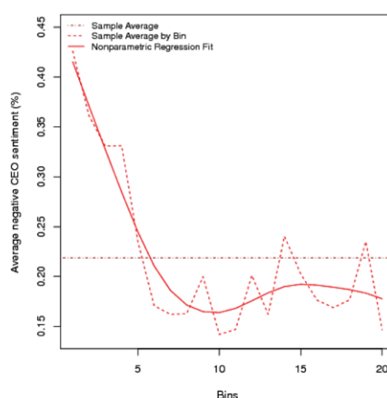
(b) Frequency plot of average negative sentiment by bin—A left-sided smirk in negative sentiment
