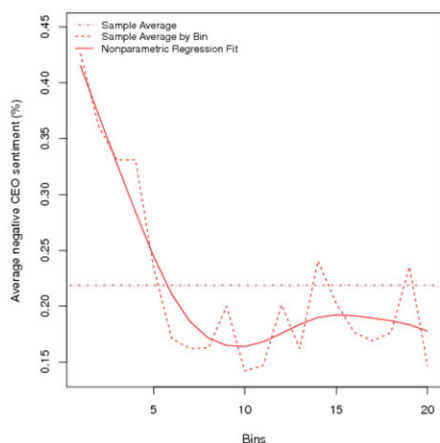
(c) Frequency plot of average negative sentiment by bin (Abrahamson-Amir)—A left-sided
