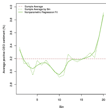
(a) Frequency plot of average positive sentiment by bin—A U-shape and smile in positive sentiment
