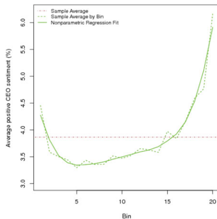
(d) Frequency plot of average net sentiment by bin—A right-sided smirk in net sentiment
