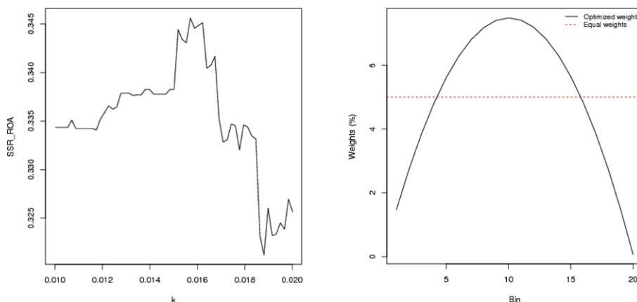
(a) Sum of squared residuals as a function of the threshold parameter kappa ( \kappa ) using Equation (16) (b) Optimized weights of intratextual net sentiment as a function of position of a word in the text
