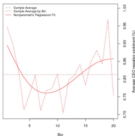
(b) Frequency plot of average negative sentiment by bin (DICTION)
