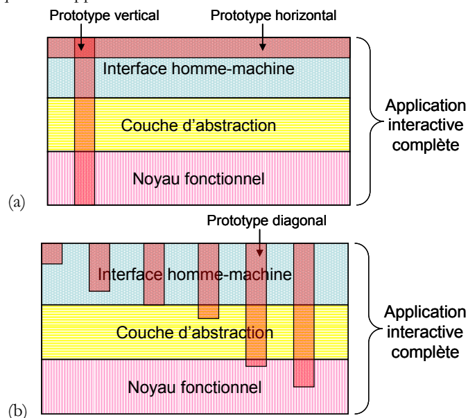
Figure 5. Prototypage vertical (a) vs. horizontal (b) (Nielsen, 1993)
