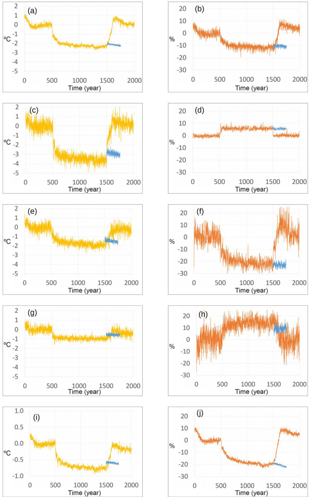
Fig. 3. a–t (next 2 pages). Simulated annual changes in surface temperature (yellow, in °C) and soil moisture (orange, in %). The reference climate is represented by year 401–500. The COMBINED experiment covers years 501–1500, with a 5Sv freshwater pulse being added in years 501–503 to the Arctic Ocean at the MacKenzie River outlet. The yellow or orange results for years 1501–2000 represent the NO_BGMF scenario, while the results of the NO_DAR scenario are provided in blue. (a,b) Central Europe, (c,d) Northeast Europe, (e,f) Western Siberia, (g,h) Southeastern North America, (i,j) Sahel region, (k,l) Southeast Asia, (m,n) Central America, (o,p) Southern South America, (q,r) Southwest Africa, (s,t) Northern Australia. (For interpretation of the references to colour in this figure legend, the reader is referred to the Web version of this article.)
