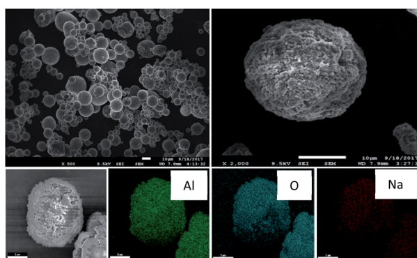
Fig. 1 (Top) SEM images of the 20 SAB samples at different magnification values (other catalysts have been analysed in SEM too and showed similar morphologies – see ESI Fig. S1†). (Bottom) SEM-EDX elemental analysis on one microparticle of 20 SAB catalyst.
