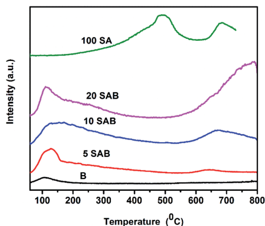
Fig. 3 CO 2 TPD profiles obtained on the catalysts. The Y-axis has been re-scaled; only the shape of the profile should be considered here.
