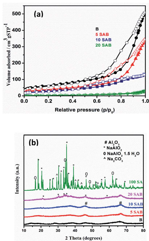
Fig. 2 (a) Nitrogen adsorption (full symbols) and desorption (empty symbols) isotherms obtained on the catalysts prepared by spray drying and calcination. (b) Powder XRD patterns.
