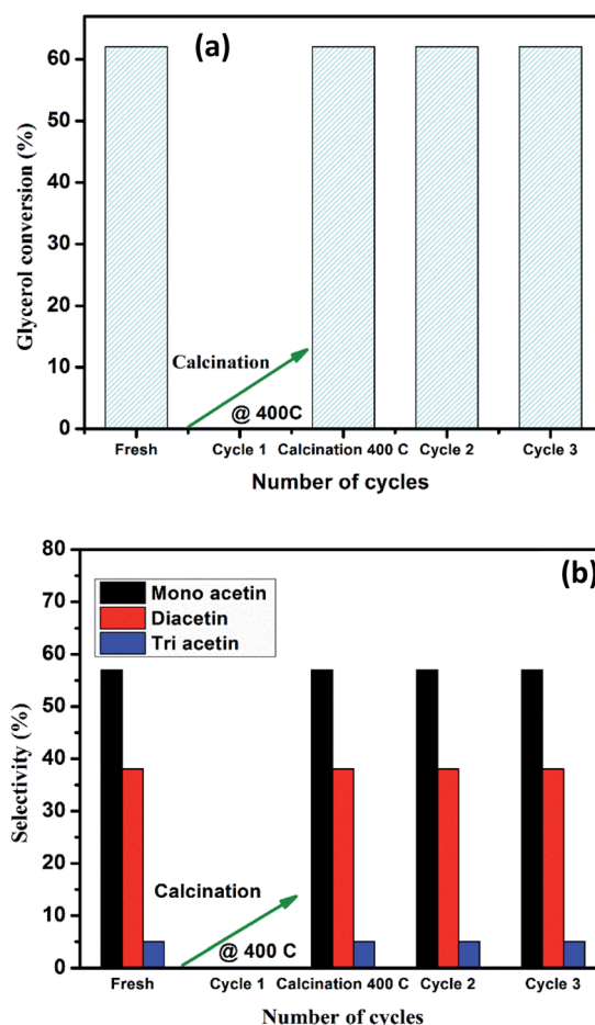
Fig. 5 Reusability studies. (a) Glycerol conversion after several rounds of recycling (with reactivation by calcination). (b) Acetins selectivity during these recycling tests. Reaction conditions: 10 mmol of glycerol, 100 mmol of methyl acetate with 0.100 g of 20 SAB at 60 °C for 1 h, after that catalyst was filtered, washed with ethanol and calcined at 400 °C for 4 h before used for next cycle.
