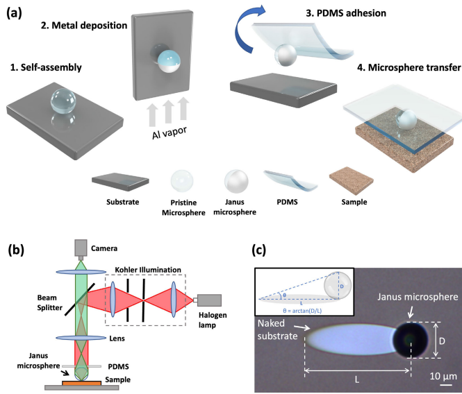
Fig. 1. (a) Illustrative drawings of the fabrication and manipulation of Janus microspheres; (b) Schematic drawing of the microsphere-assisted microscopic imaging system; (c) Optical picture of a Janus microsphere after Al deposition.
