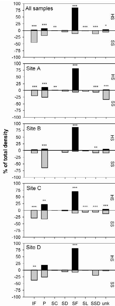
Figure 11. Contribution of the different trophic groups to total density. The soft sediment samples selected around hard substrate sites are within a circle of 5 nautical miles. On hard substrates, the dominant species Jassa herdmani is excluded from calculation. IF: interface feeder, P: predator, SC: scavenger, SD: deposit feeder, SF: suspension feeder, SL: sand licker, SSD: subsurface deposit feeder, Unk: unknown type. *** p<0.001, ** p<0.01, * p<0.05 (significance level of a Mann-Whitney U test).
