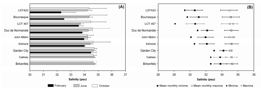
Figure 2. Water salinity on the nine shipwrecks. (A) Mean monthly values (+s.d.) for February, June and October. (B) Mean ( \pm s.d.) monthly minima and maxima. Period covered: 1993-2006.
