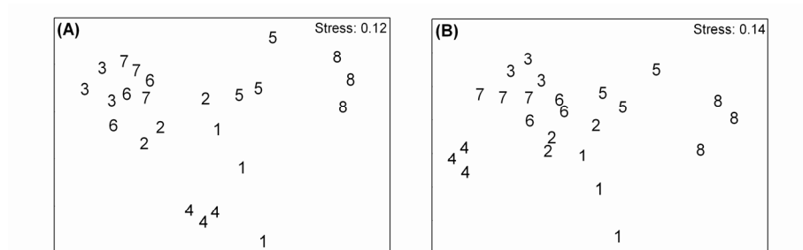
Figure 8. non-Metric Multidimensional Scaling based on Bray-Curtis similarity from \sqrt{\sqrt{}} abundance data (A) and presence/absence data (B). 1: December 2003, 2: April 2004, 3: July 2004, 4: October 2004, 5: March 2005, 6: June 2005, 7: August 2005, 8: October 2005.
