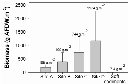
Figure 8. Biomass on hard substrates (sites A to D) and soft sediments.
