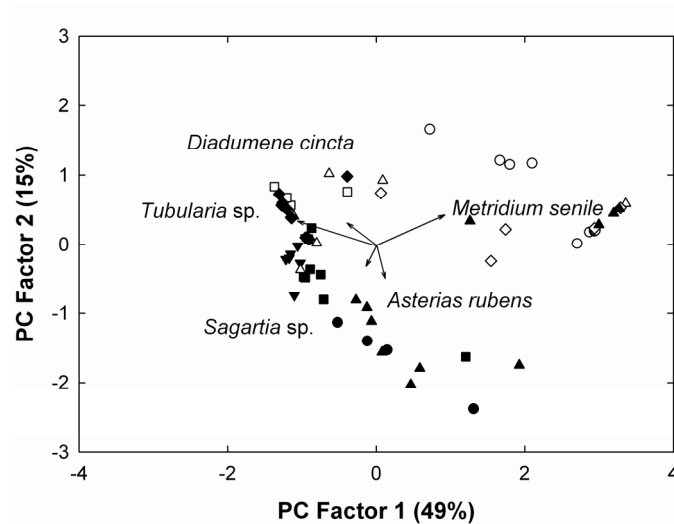
Figure 11. Principal Components Analysis biplot of the epifauna cover data (on covariance matrix, double-root-transformed data). Only the main variables and the sites with \Sigma \text{Cos}^2 \geq 0.40 are represented. Sites symbolism: ■ Bourrasque, □ LST 420, ● John Mahn, ○ Duc de Normandie, ◆ Birkenfels, ◇ Kilmore, ▲ Callisto, △ LCT 457, x Garden City.
