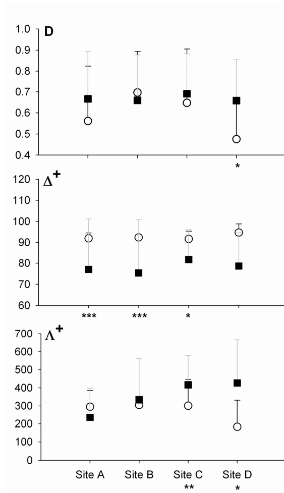
Figure 7. Diversity index comparison of hard substrate (○) with selected soft sediment (■) samples around hard substrates (distance: circle of 5 nautical miles, number of samples: site A (38), B (14), C (90), D (118)). Values are mean values + standard error. D is the Simpson index; \Delta^+ is the average taxonomic distinctness; \Lambda^+ is the variation in taxonomic distinctness. Significant difference between means tested with Monte Carlo permutation (999 randomizations) (* p < 0.05 , ** p < 0.01 , *** p < 0.001 ).
