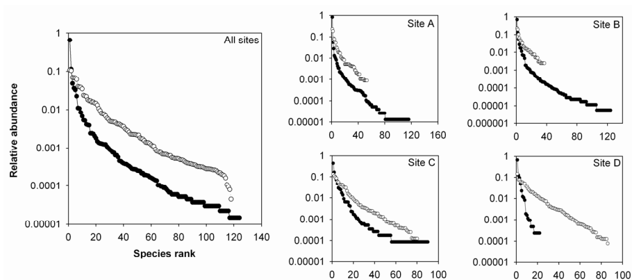
Figure 3. Rank/abundance plot based on count of species on hard substrates (●) and selected soft sediments (○) around hard substrate sites (distance: circle of 5 nautical miles, number of samples: site A (38), B (14), C (90), D (118))
