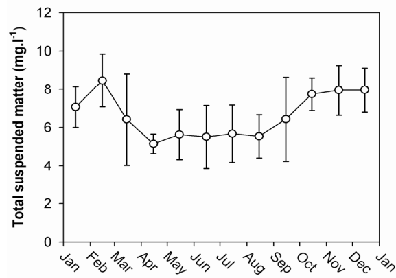
Figure 4. Mean monthly total suspended matter ( \pm s.d.) on the Kilmore obtained from Modis satellite imagery for the period July 2002 to October 2005 (Number of observations = 199).
