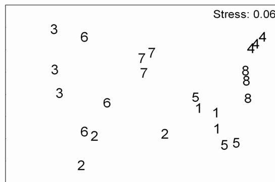
Figure 9. non-Metric Multidimensional Scaling based on Euclidean distances from \sqrt{\sqrt{}} biomass data. 1: December 2003, 2: April 2004, 3: July 2004, 4: October 2004, 5: March 2005, 6: June 2005, 7: August 2005, 8: October 2005.
