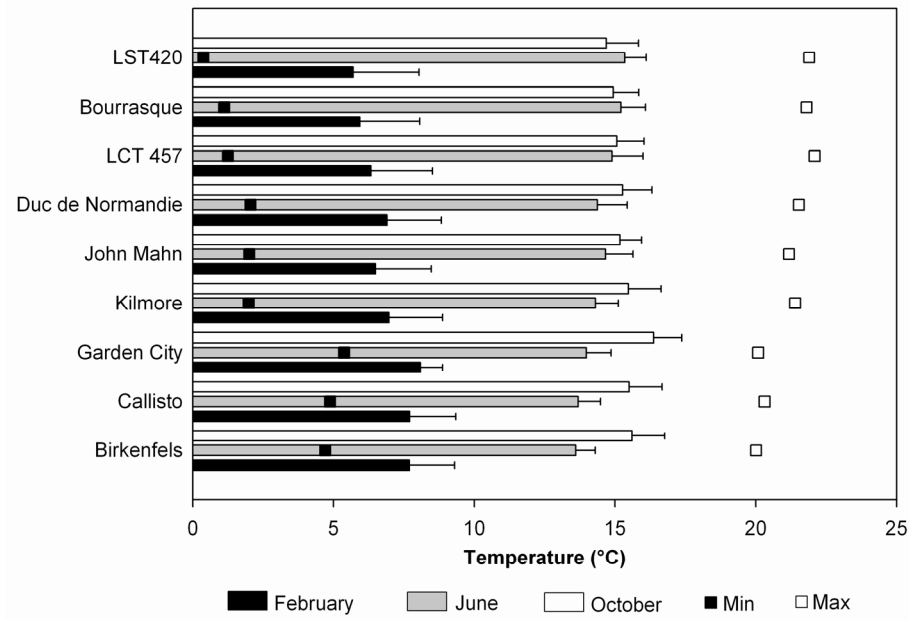
Figure 1. Water temperature on the nine shipwrecks. The mean monthly values (+s.d.) for February, June and October are presented together with minimal and maximal observed temperature. Period covered: 1993-2006.
