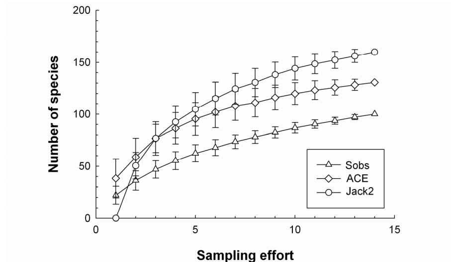
Figure 2. Species accumulation curves. Estimators of the species richness are the total number of observed species (Sobs), the Abundance based Coverage Estimator (ACE) and the Jackknife 2 Estimator of true richness. Plotted values are mean \pm SD of 100 estimates based on 100 randomizations.
