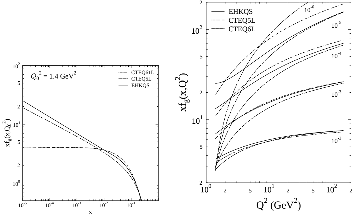
Fig. 4: Left: initial gluon distributions at Q_0^2 = 1.4 \text{ GeV}^2 . Right: evolution of gluon distributions for several fixed values of x shows that the effect of the nonlinear terms vanishes as Q^2 increases.
