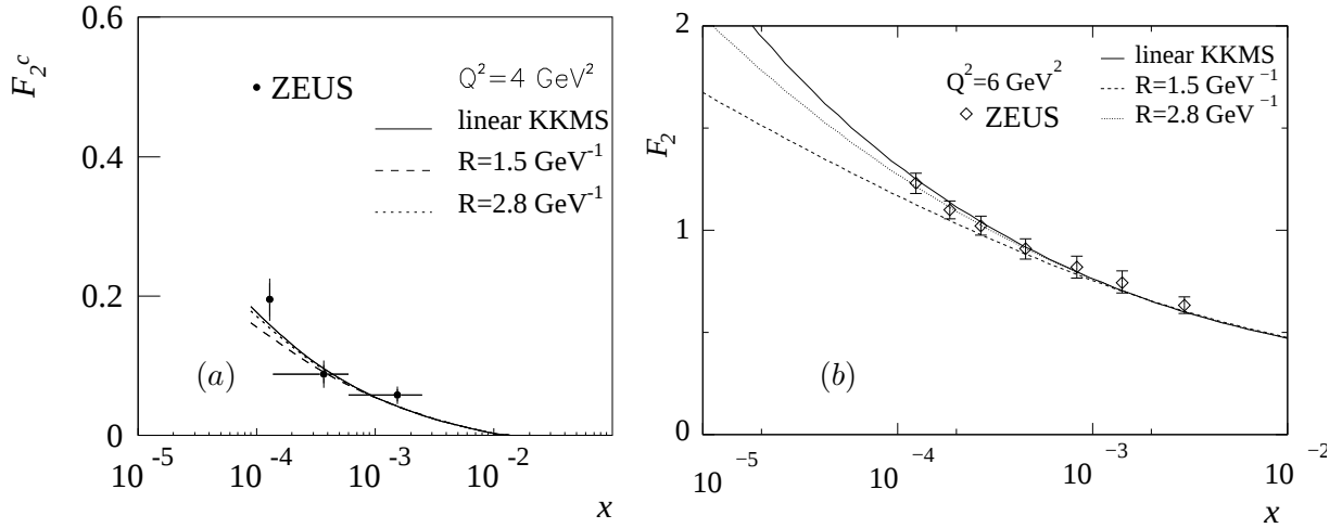
Fig. 6: The charm structure function, F_2^c , [61] at Q^2 = 4 \text{ GeV}^2 (a) and F_2 [64] at Q^2 = 6 \text{ GeV}^2 (b) obtained for KKMS evolution with different values of R .
