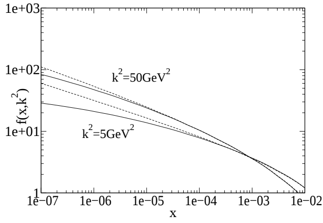
Fig. 5: The unintegrated gluon distribution obtained from Eq. (8) as a function of x for different values of k_T^2 . The solid lines correspond to the solution of the nonlinear equation with R = 2.8 \text{ GeV}^{-1} while the dashed lines correspond to the linear part.
