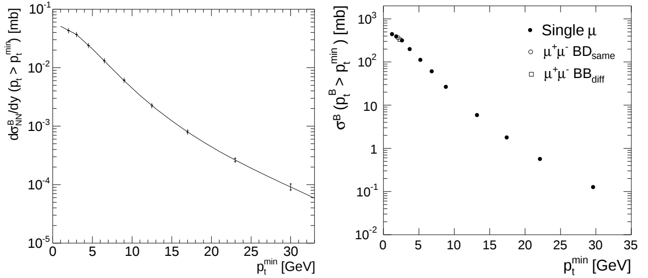
Fig. 4: B production cross section vs. p_T^{\min} reconstructed by ALICE in 10^7 central Pb–Pb events. Left: d\sigma_{\text{NN}}^{\text{B}}/dy at y = 0 (normalized to one nucleon–nucleon collision) from single electrons in |\eta| < 0.9 ; statistical (inner bars) and quadratic sum of statistical and p_T -dependent systematic errors (outer bars) are shown; a 9% normalization error is not shown. Right: \sigma^{\text{B}} integrated in 2.5 < y^{\text{B}} < 4 (not normalized to one nucleon–nucleon collision) from single muons and di-muons in 2.5 < \eta < 4 ; only (very small) statistical errors shown.
