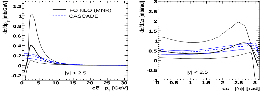
Fig. 9: Q\bar{Q} correlations for charm at LHC: p_T of the c\bar{c} pair (left) and azimuthal angle \Delta\phi between the c and the \bar{c} (right). For both cross sections, the following kinematic cuts are applied: |Y^c| < 2.5 , |Y^{\bar{c}}| < 2.5 , p_T^c > 3 GeV, p_T^{\bar{c}} > 6 GeV.
