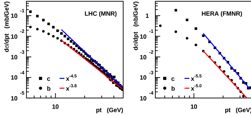
Fig. 1: Power-law fits to the heavy quark p_T distributions at LHC (left) and HERA (right) obtained with the NLO programs MNR and FMNR. The resulting exponents are N = 4.5/3.8 for charm/beauty at LHC and N = 5.5/5.0 for c/b at HERA.
