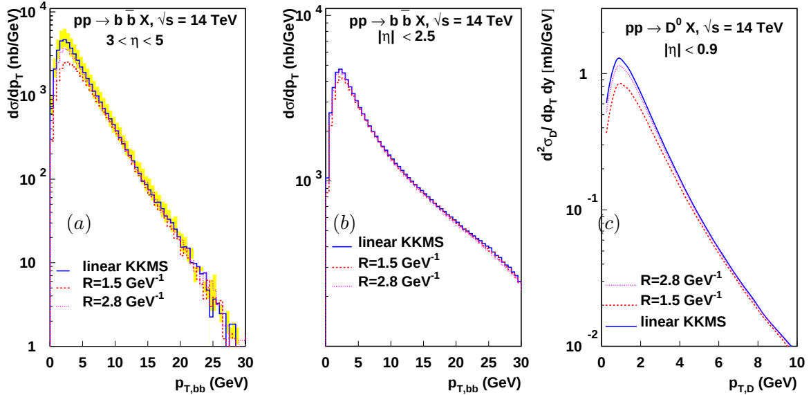
Fig. 9: (a) and (b) show b\bar{b} production as a function of pair p_T without cuts in 3 < |\eta| < 5 (a) and in the ATLAS/CMS acceptance (b). The D^0 meson p_T distribution in the ALICE acceptance is shown in (c).
