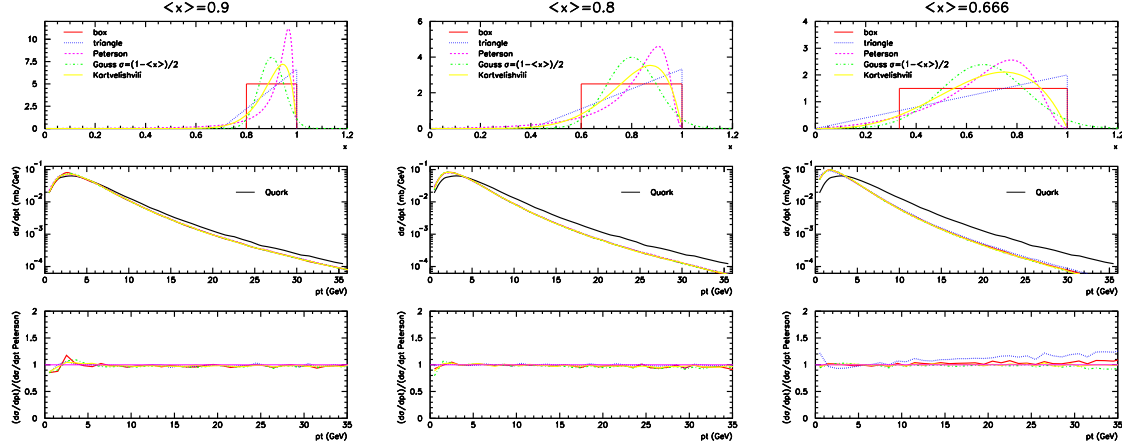
Fig. 2: Effect of the convolution of the heavy quark transverse momentum distribution with different test functions for different values of the non-perturbative FF \langle x \rangle = 0.9 (left), 0.8 (center), 0.666 (right). For each \langle x \rangle , the upper plot shows the test functions, the middle plot shows the perturbative p_T distribution obtained with the MNR program for beauty at LHC and the hadron p_T distributions after the convolution with the test functions. The lower plot shows the ratio of the different hadron p_T distributions to the result obtained with the Peterson one.
