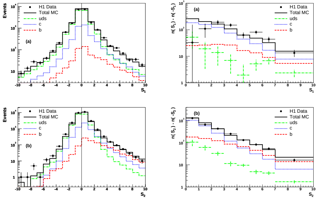
Fig. 7: Upper left: significance S_1 = \delta/\sigma(\delta) distribution per event for events that contain one selected track associated to the jet axis. Lower left: significance S_2 = \delta/\sigma(\delta) distribution per event of the track with the second highest absolute significance for events with \geq 2 selected tracks associated to the jet. Right: S_1 and S_2 distributions after subtracting the negative bins in the S_1 and S_2 distributions from the positive.
