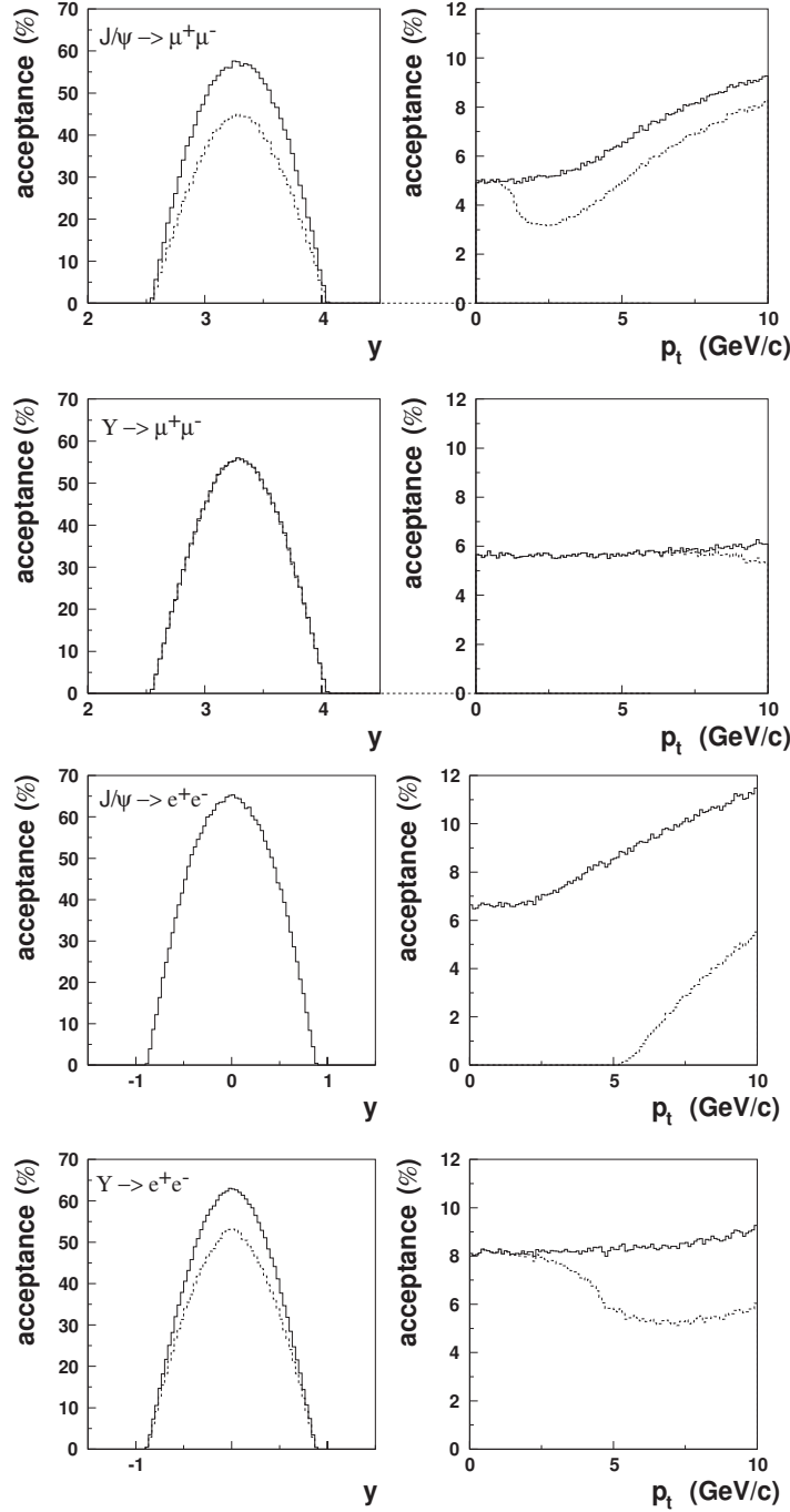
Fig. 6: Acceptance for J/\psi and \Upsilon as a function of y and p_T for measurements in the di-muon channel and di-electron channels. To give an idea of the effect of the trigger, the acceptances are shown without (solid) and with (dashed) a sharp cut on the transverse momentum of single muons of 1 GeV/c (2 GeV/c) for J/\psi ( \Upsilon ) and for single electrons of 3 GeV.
