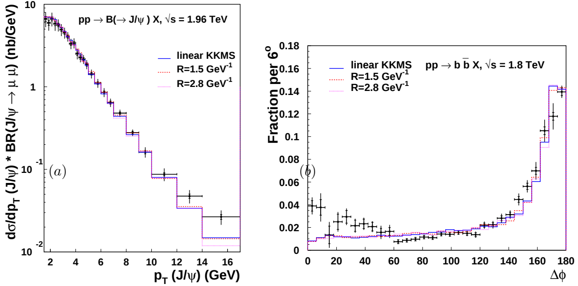
Fig. 7: Bottom production, measured by CDF, is compared to predictions using CASCADE with linear and nonlinear KKMS evolution, including two values of R . (a) The p_T distribution of B meson decays to J/\psi . (b) The azimuthal angle, \Delta\phi , distribution of b\bar{b} pair production smeared by the experimental resolution.
