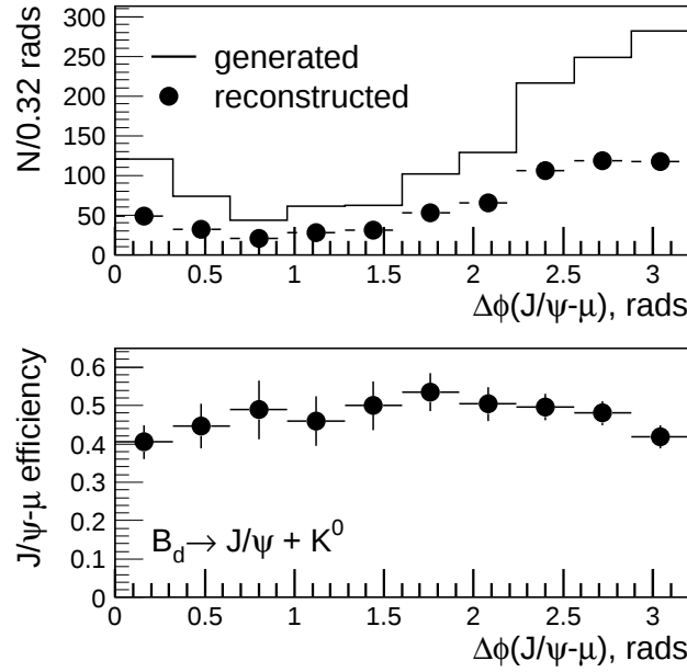
Fig. 5: Distribution of the opening angle \Delta\phi(J/\psi-\mu) between the J/\psi from the decay B_d \rightarrow J/\psi K^0 and the muon coming from the associated B hadron decay to muon, both direct b \rightarrow \mu and indirect b \rightarrow c \rightarrow \mu .
