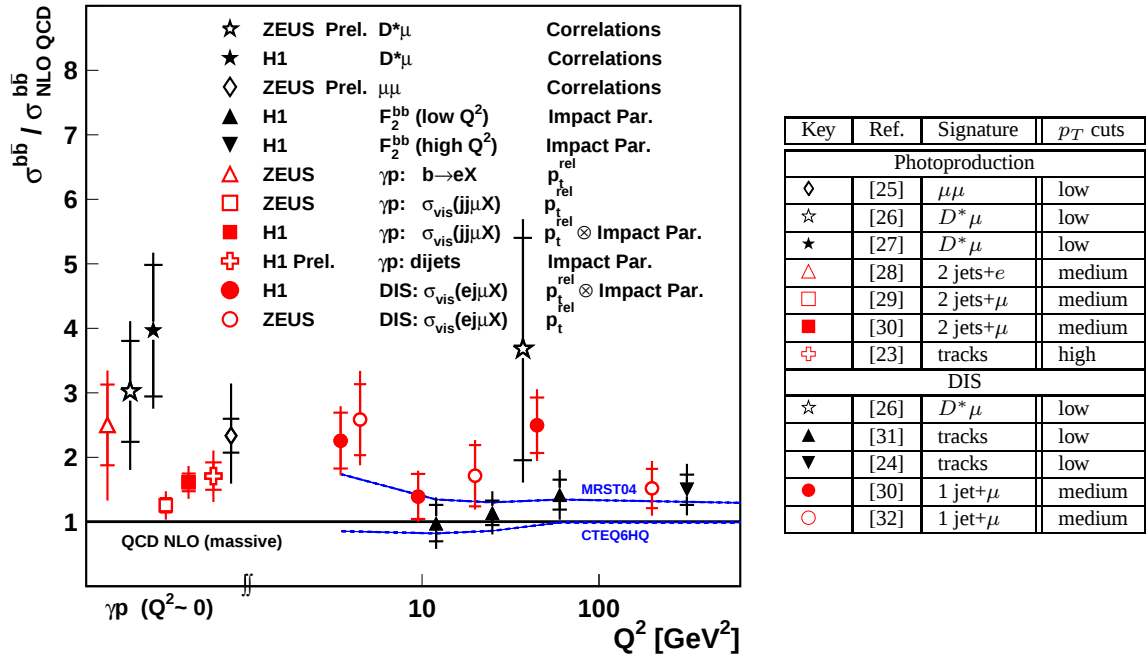
Fig. 9: Ratio of beauty production cross section measurements at HERA to NLO QCD predictions in the massive scheme as function of the photon virtuality Q^2 . Measurements with low p_T cuts are shown in black, while measurements with medium or high p_T cuts are shown in red/grey. For more details see Table. The predictions from the VFNS NLO calculations by MRST and CTEQ for the DIS kinematic regime Q^2 > 2 \text{ GeV}^2 are also shown (valid for comparison with the black low threshold points). Since theoretical errors are different for each point, they are not included in this plot.
