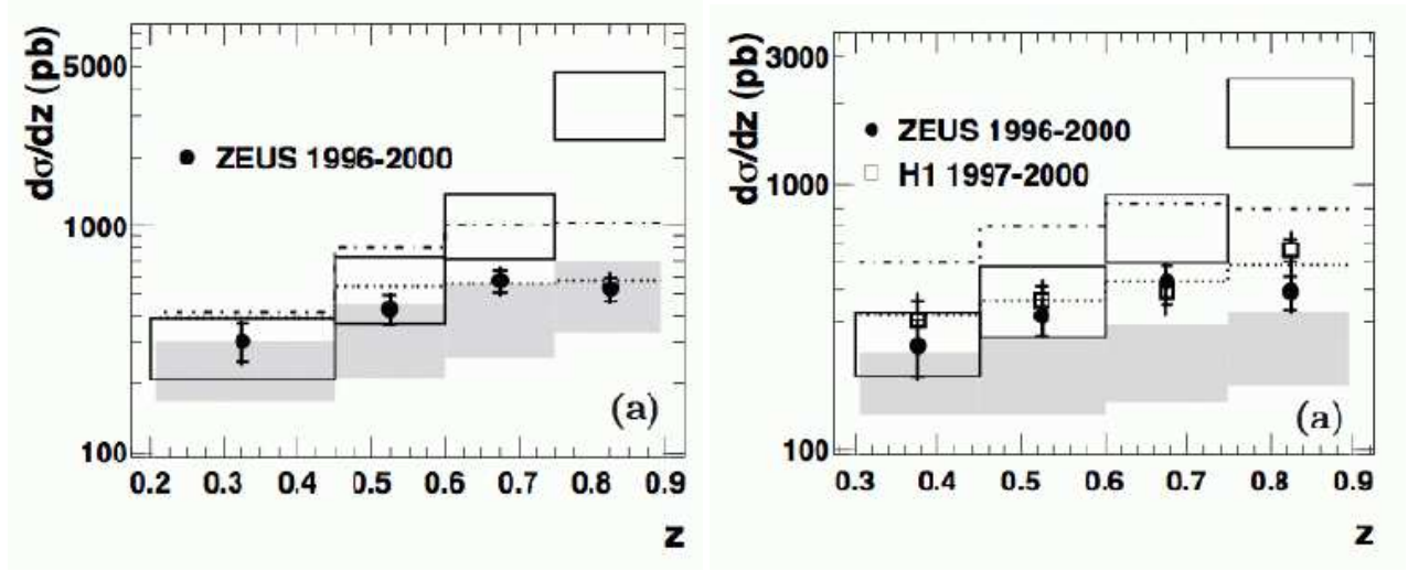
Fig. 13: Differential cross sections d\sigma/dz without (left) and with (right) a cut on p_{t,\psi}^{*2} > 1 GeV. The data are compared to the NRQCD calculation (CS+CO, open band), the color-singlet contribution (CS, shaded band), with a prediction in the k_t factorization approach assuming the CSM (dotted line) and with the Monte Carlo generator CASCADE (dash-dotted line).
