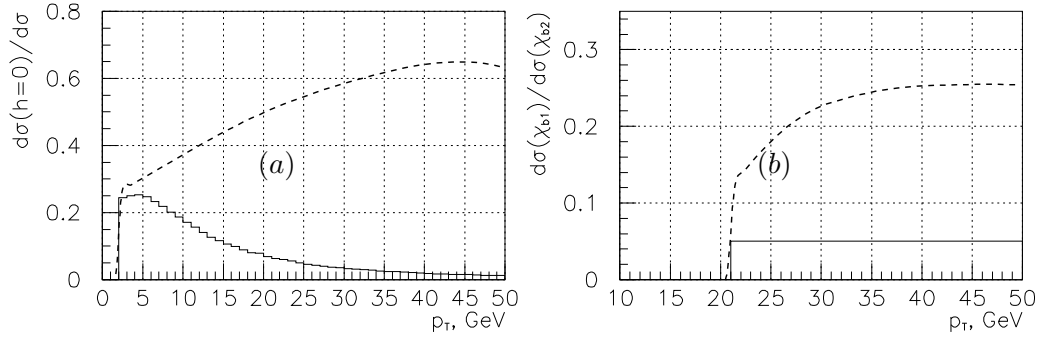
Fig. 9: Predictions of different theoretical approaches for quarkonium production. In (a) the fraction of longitudinally polarized \Upsilon mesons is shown: solid histogram - collinear parton model, singlet + octet; dashed - k_t -factorization with KMS u.g.d.. In (b) the ratio of the production rates \chi_{b1}/\chi_{b2} is shown: solid histogram - collinear parton model, singlet + octet; dashed - k_t factorization with KMS u.g.d.
