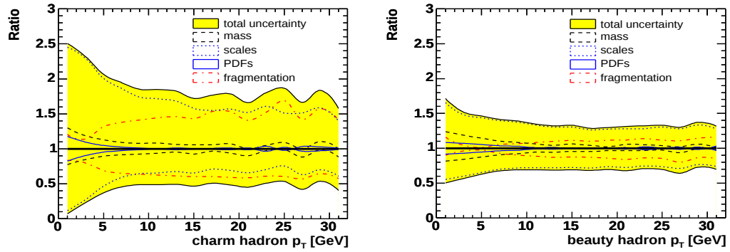
Fig. 8: Breakdown of the different components of the uncertainty on d\sigma/dp_T for charmed (a) and beauty (b) hadrons at LHC as obtained from MNR. The plots show the ratio of the upper/lower side of each uncertainty to the nominal value. The following sources of uncertainty are shown: quark mass ( m_Q ), parton density parametrisation (PDF), fragmentation parameter and the perturbative uncertainty from scale variations.
