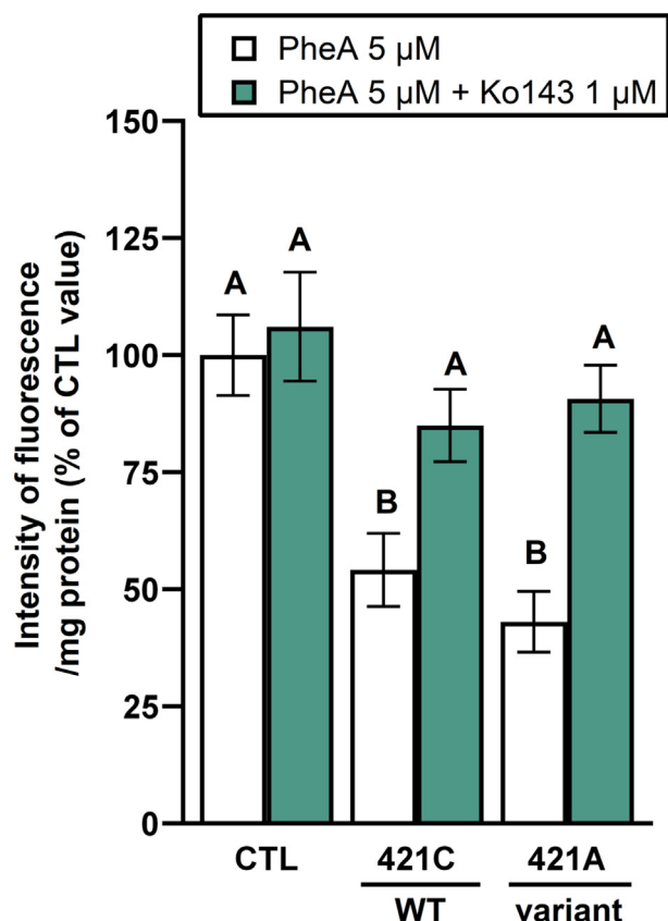
Fig. 3. Impact of ABCG2 transporter on the cellular accumulation of pheophorbide A (PheA). Cell-associated fluorescence of PheA (5 µM) after 1 hour of incubation in control conditions or the presence of the ABCG2 inhibitor Ko143 (1 µM) in HEK control (CTL), HEK wild type (421C), and HEK variant (421A). The HEK control (CTL) in each panel corresponds to the clone used to overexpress the corresponding transporter and transfected by the corresponding empty vector. Intensity of fluorescence is reported in arbitrary units. Results are reported as mean ± SEM ( n = 9 ) expressed as a percentage of the CTL value (100%). Statistical analysis: 2-way ANOVA with Tukey post hoc test, comparison between all conditions in all cell lines. Values with different letters are statistically different from each other ( P < .05 ). ABCG2, ATP-binding cassette subfamily G member 2; HEK, human embryonic kidney.
