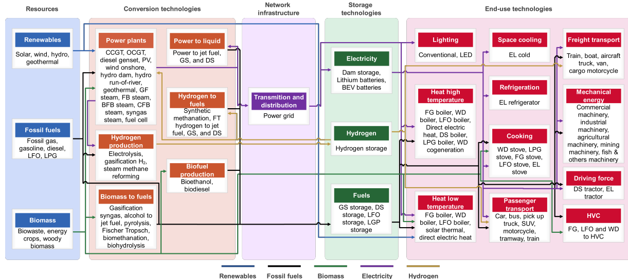
Figure 3: Simplified representation of energy system model.
