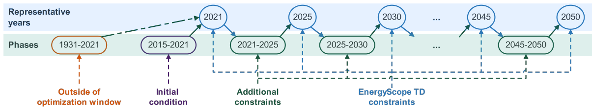
Figure 2: The methodology for the pathway is based on representative years (indicated by blue circles), during which the EnergyScope TD model is utilized. Additionally, the approach incorporates linking constraints (highlighted in green boxes), an initial condition (purple box), and the phases outside the optimization window (orange box).
